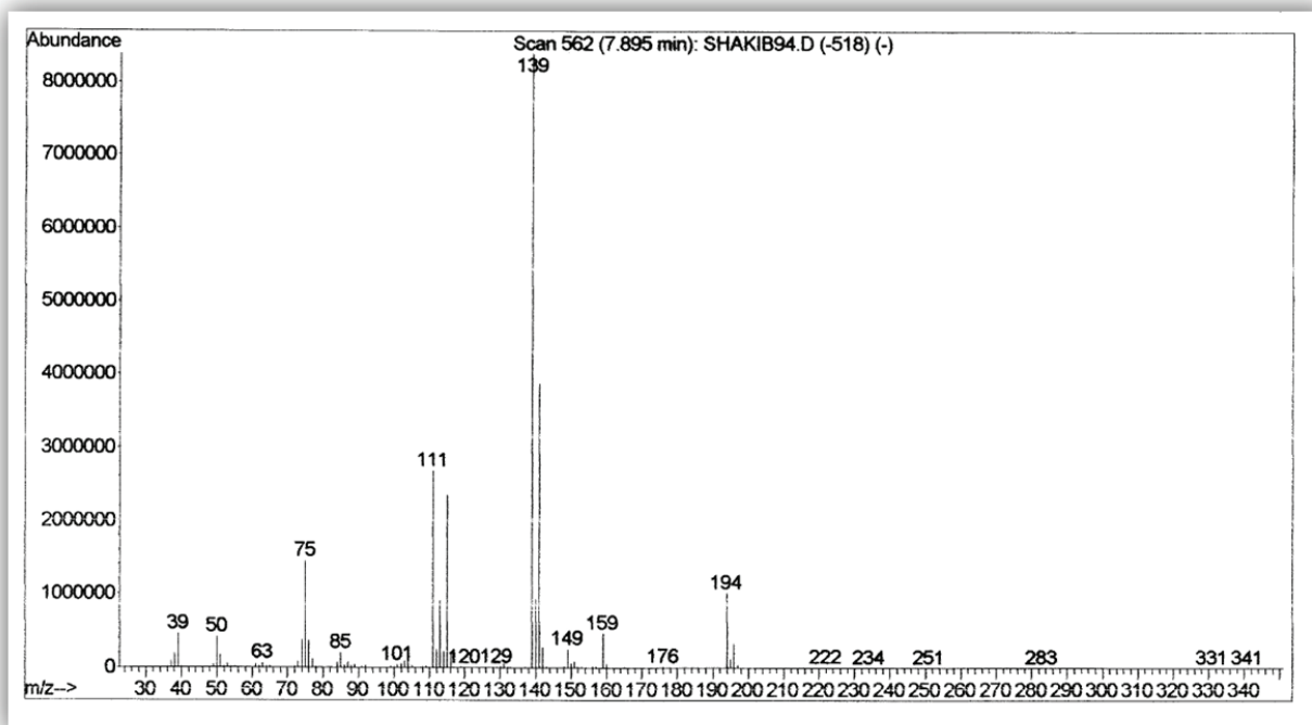
Mass spectrum of 4
