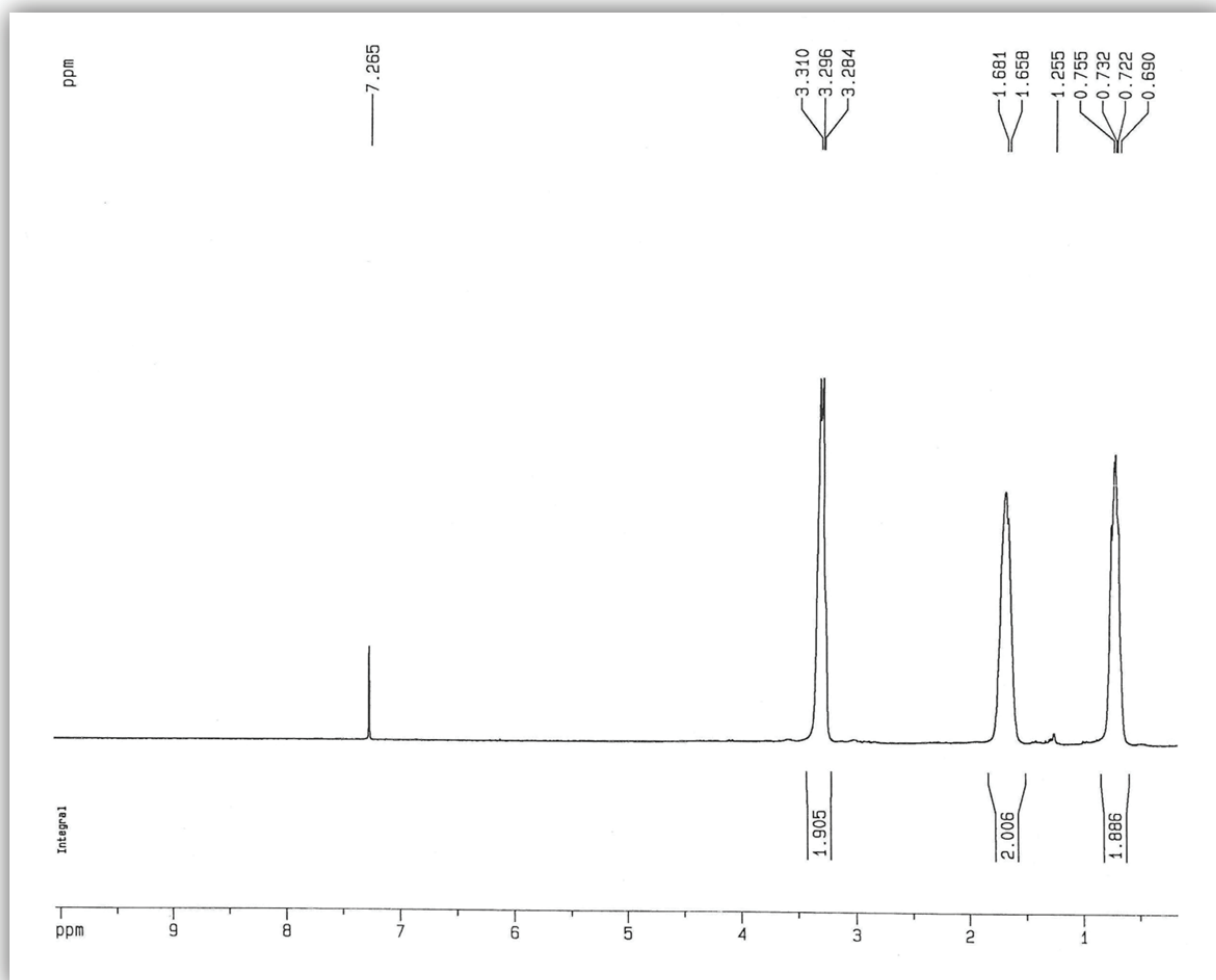
^1\text{H} NMR spectrum of POSS-(N 3 ) 8 3
