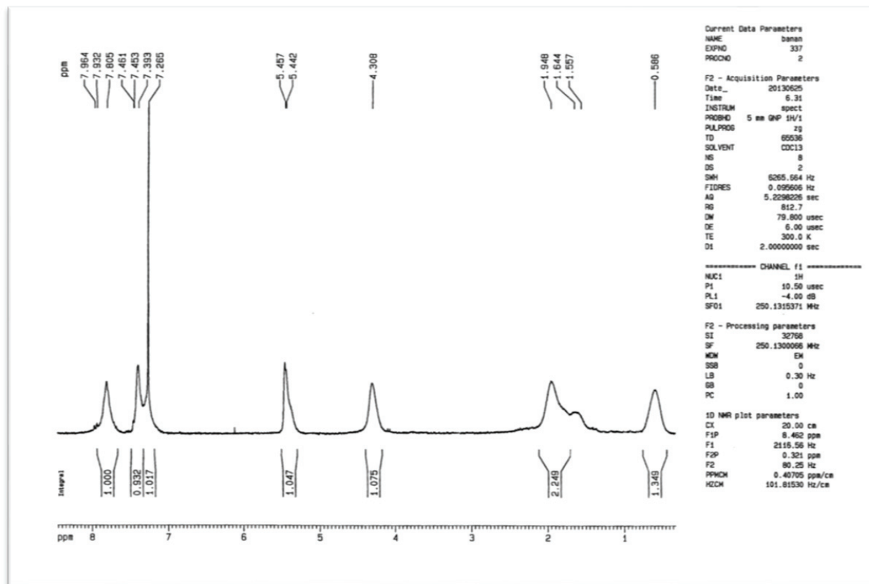
^1\text{H} NMR spectrum of 5
