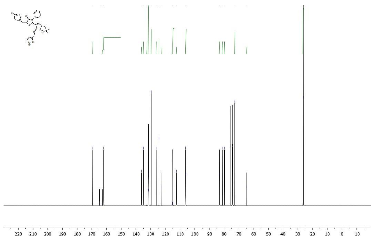
^{13}\text{C} -NMR Spectrum of Compound: 9a
