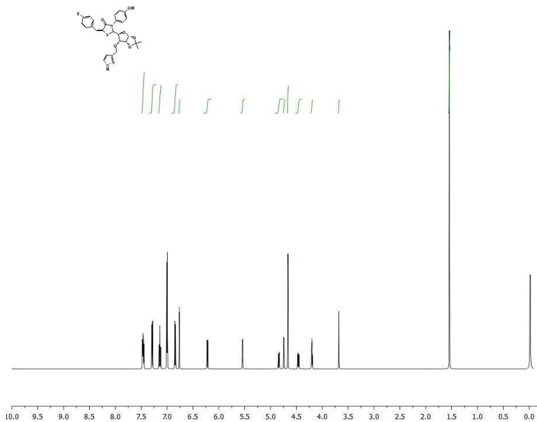
1 H-NMR Spectra of Compound: 9g
