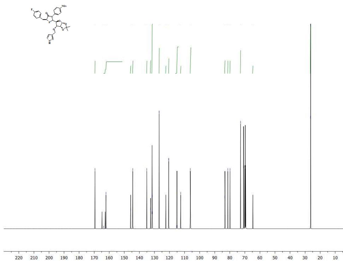
^{13}\text{C} -NMR Spectrum of Compound: 9c
