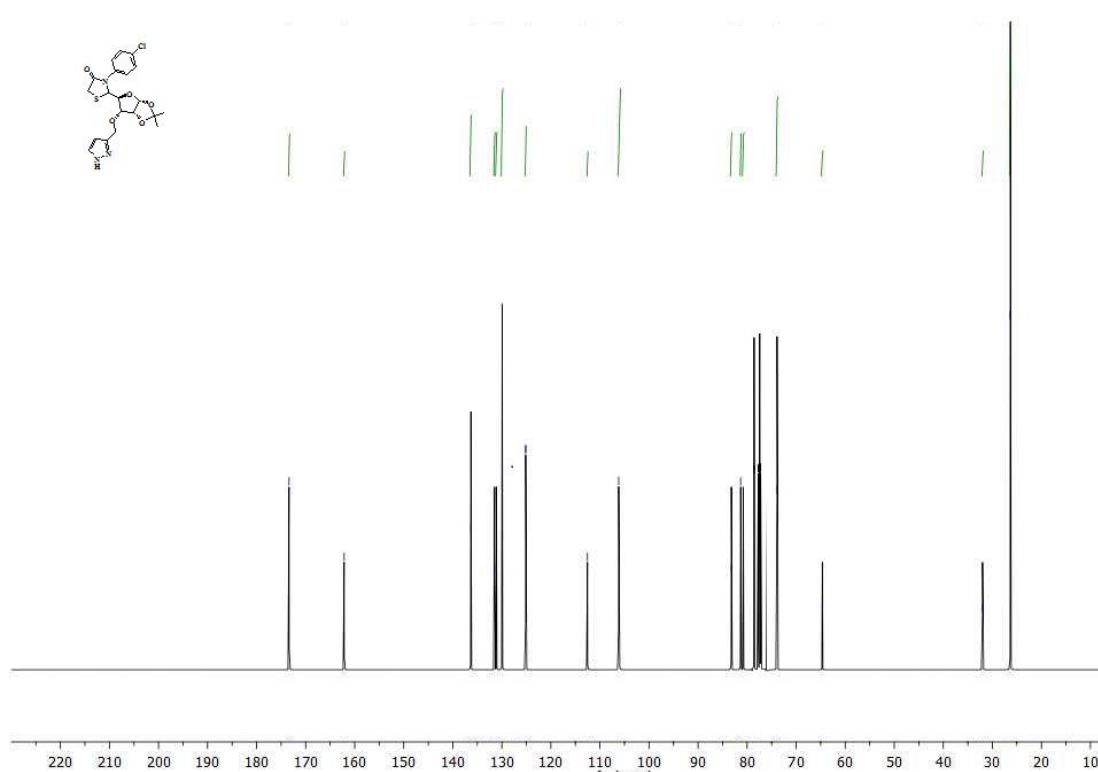
^{13}\text{C} -NMR Spectrum of Compound: 8b
