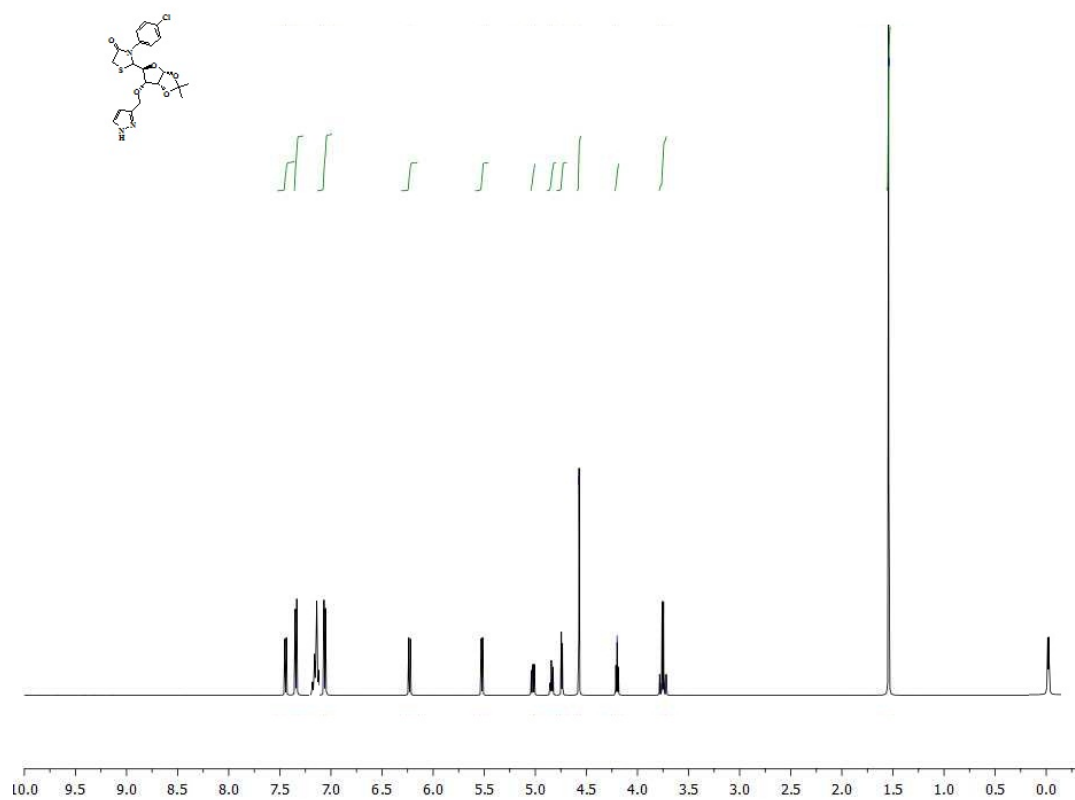
^1\text{H} -NMR Spectra of Compound: 8b
