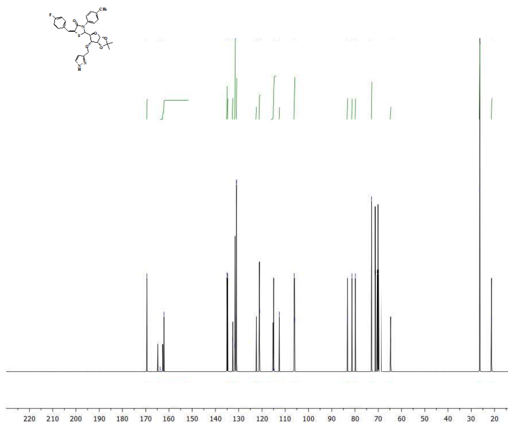
13 C-NMR Spectrum of Compound: 9e
