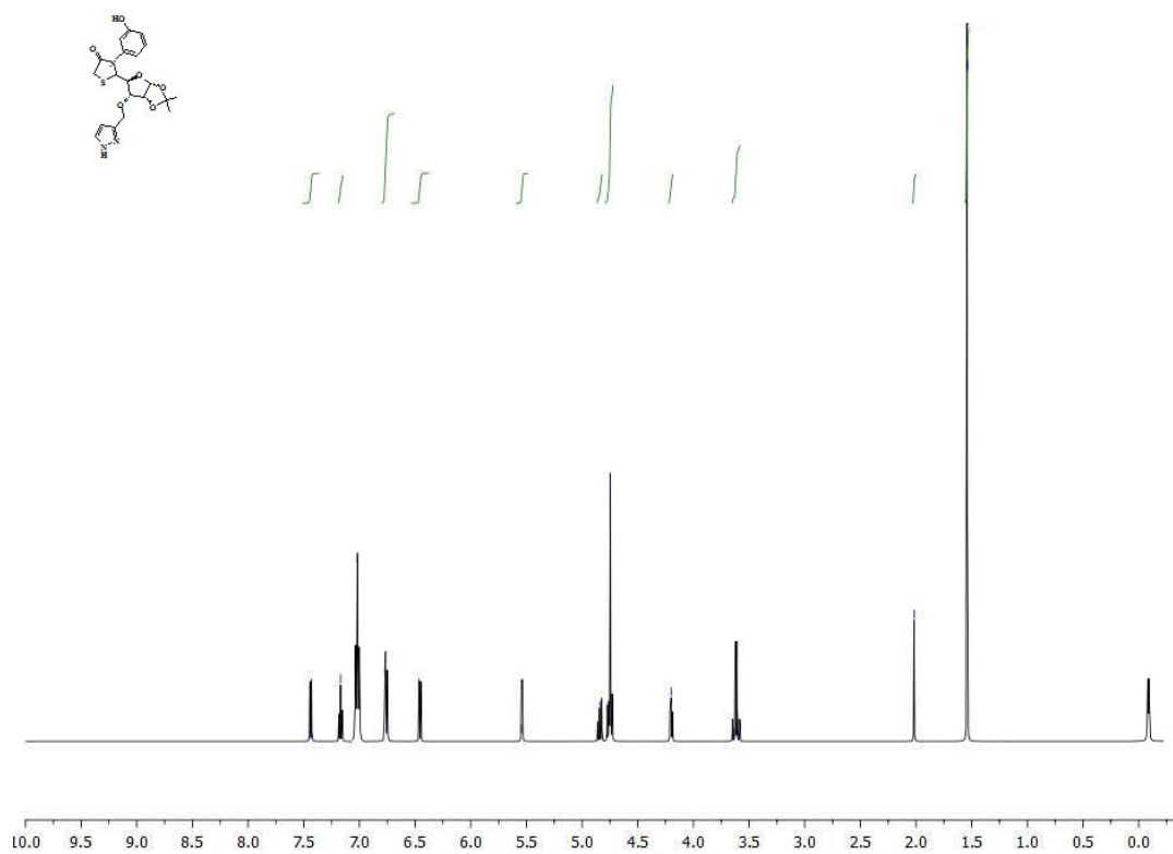
^1\text{H} -NMR Spectra of Compound: 8f
