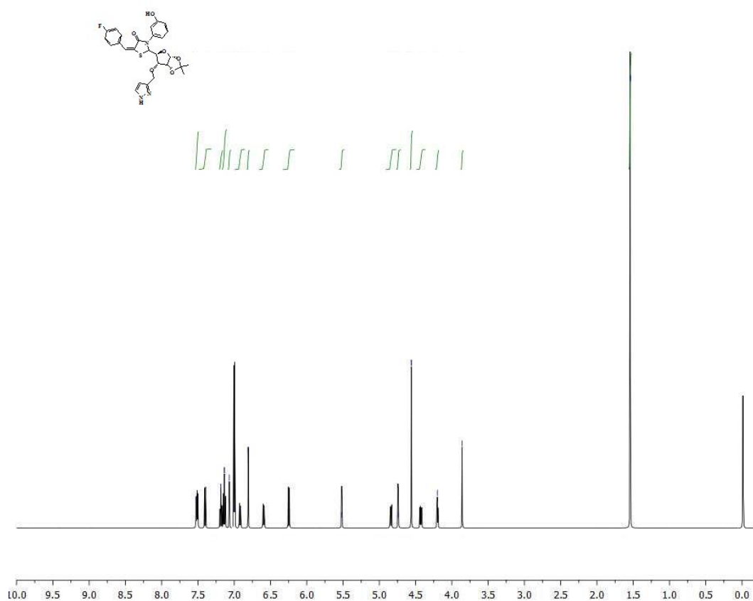
1 H-NMR Spectra of Compound: 9f
