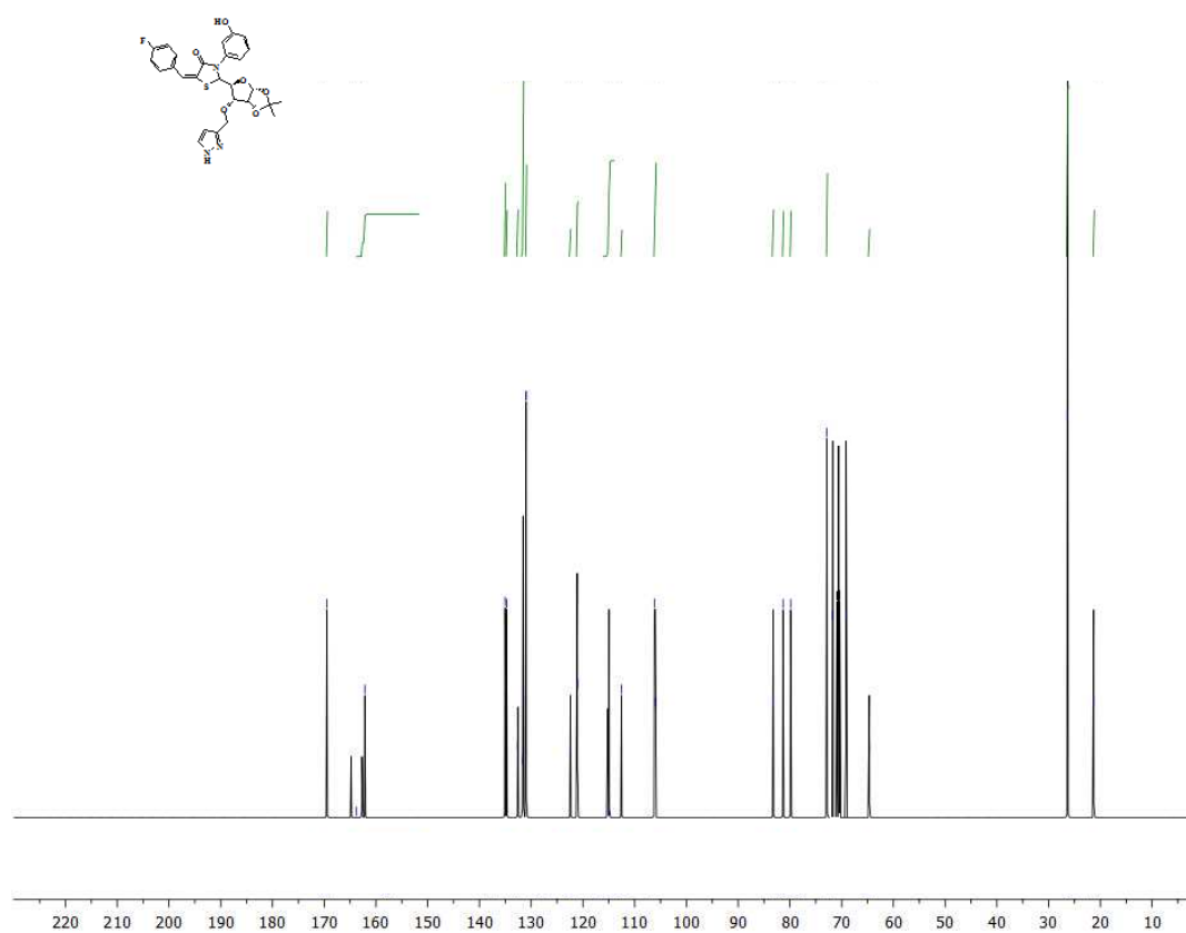
^{13}\text{C} -NMR Spectrum of Compound: 9f
