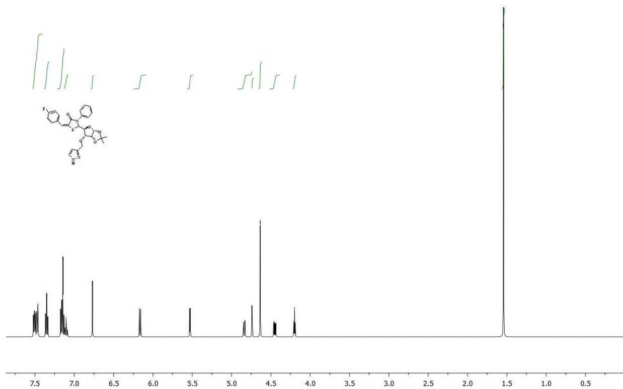
1 H-NMR Spectra of Compound: 9a
