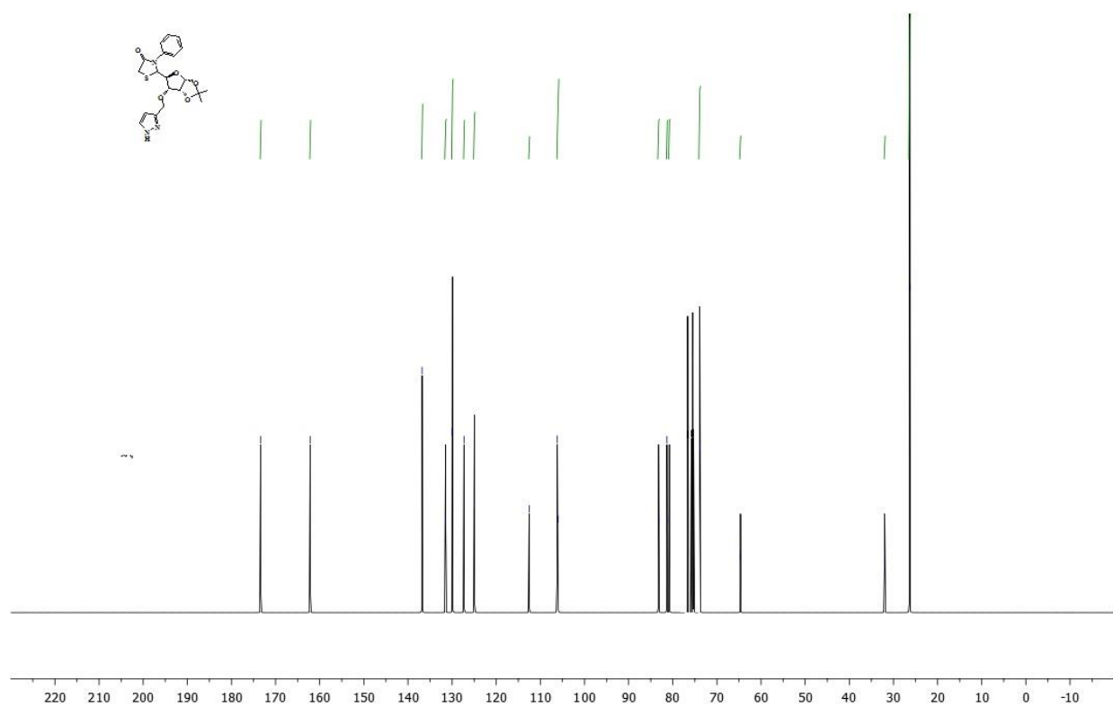
^{13}\text{C} -NMR Spectrum of Compound: 8a
