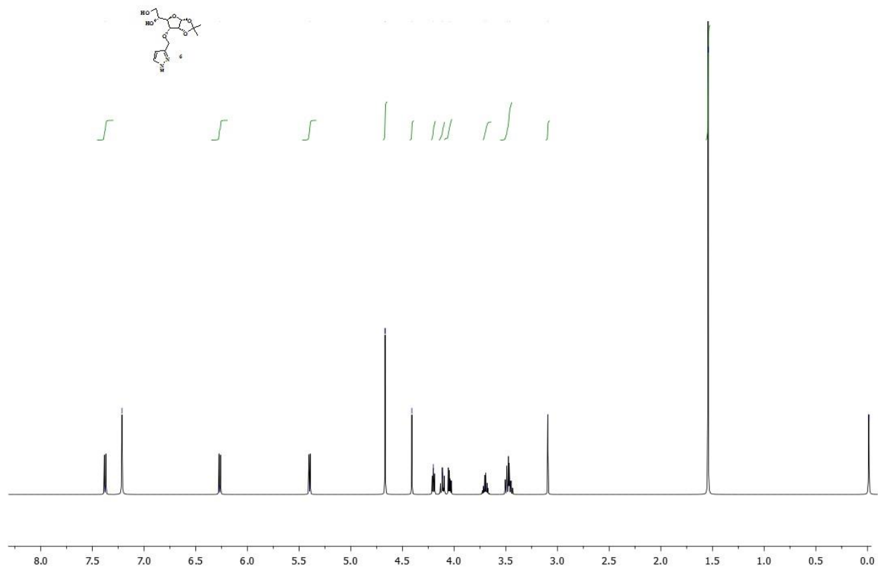
^1\text{H} -NMR Spectra of Compound: 6
