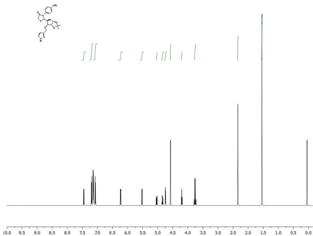
^1\text{H} -NMR Spectra of Compound: 8e
