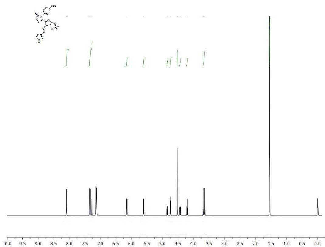
^1\text{H} -NMR Spectra of Compound: 8c
