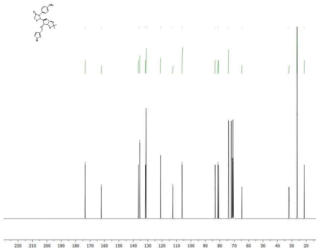
13 C-NMR Spectra of Compound: 8e
