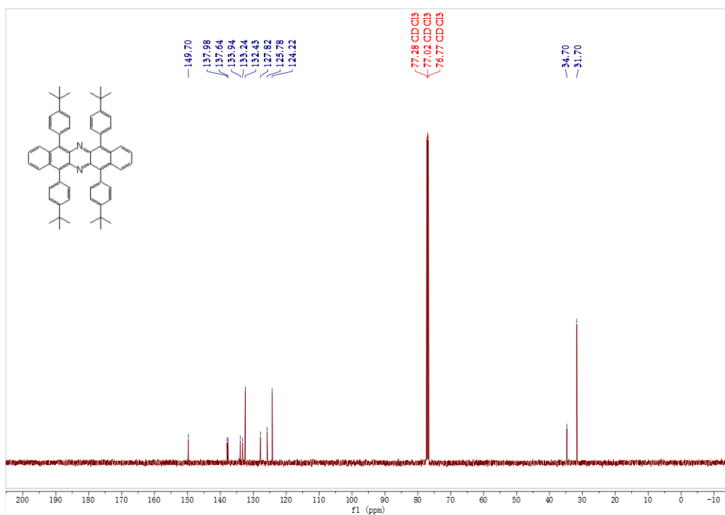
Figure S47. 13 C NMR spectrum of the compound of 7e
