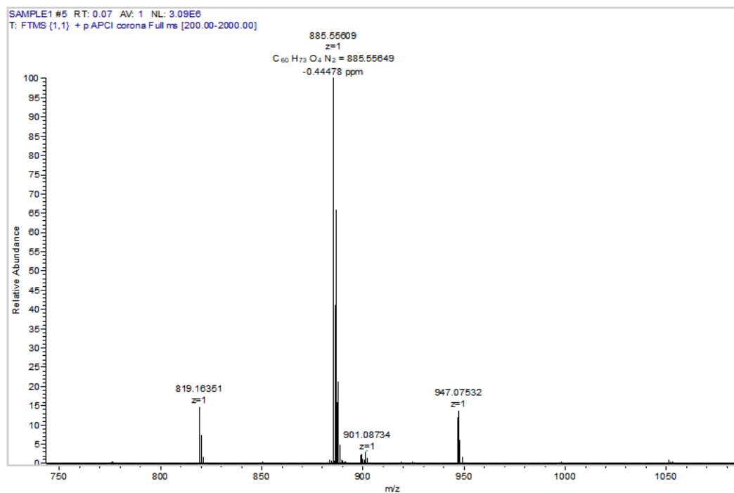
Figure S23. HRMS (APCI) spectrum of the compound of 3g
