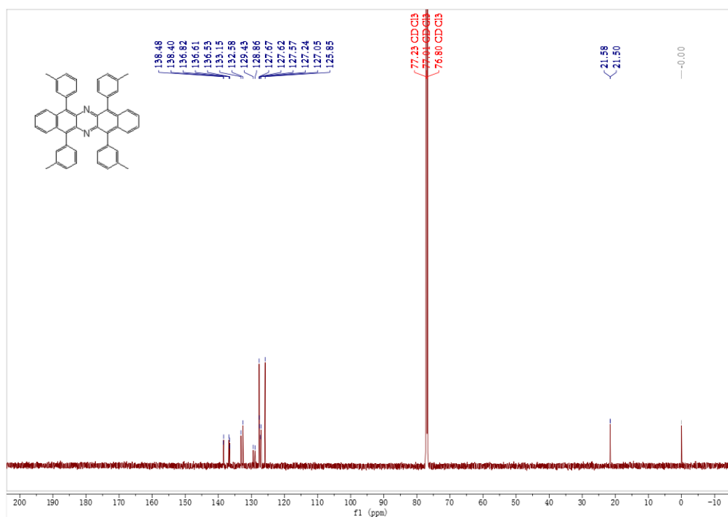
Figure S38. 13 C NMR spectrum of the compound of 7c
