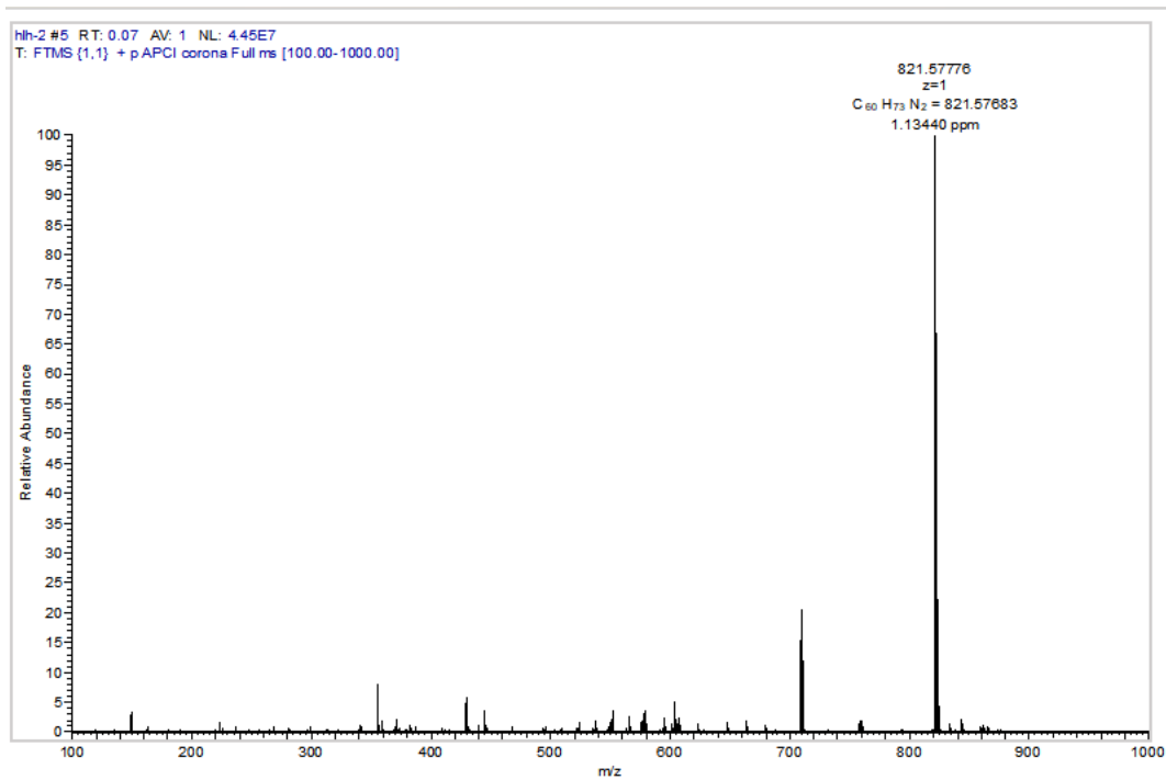
Figure S21. HRMS(APCI) spectrum of the compound of 3f
