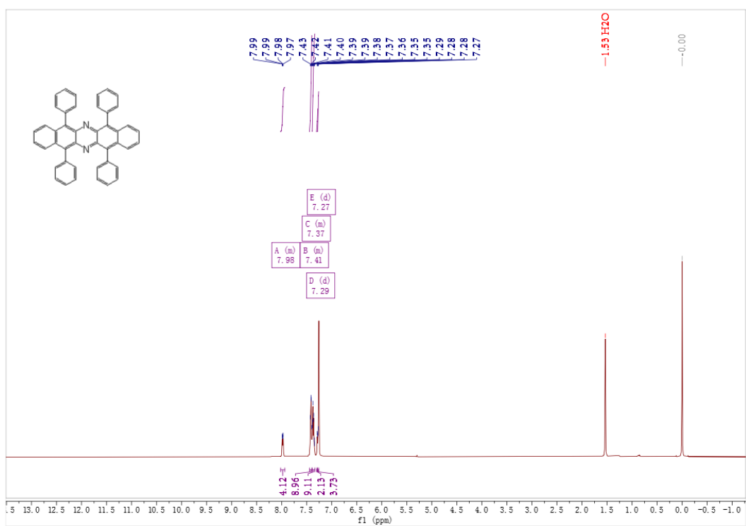
Figure S30. 1 H NMR spectrum of the compound of 7a
