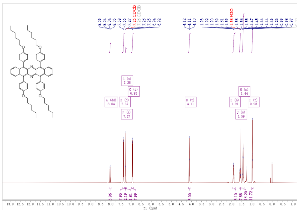
Figure S58. 1 H NMR spectrum of the compound of 7g
