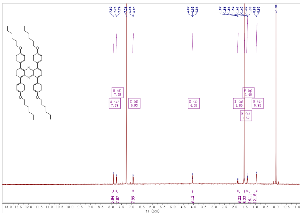
Figure S22. ^1\text{H} NMR spectrum of the compound of 3g
