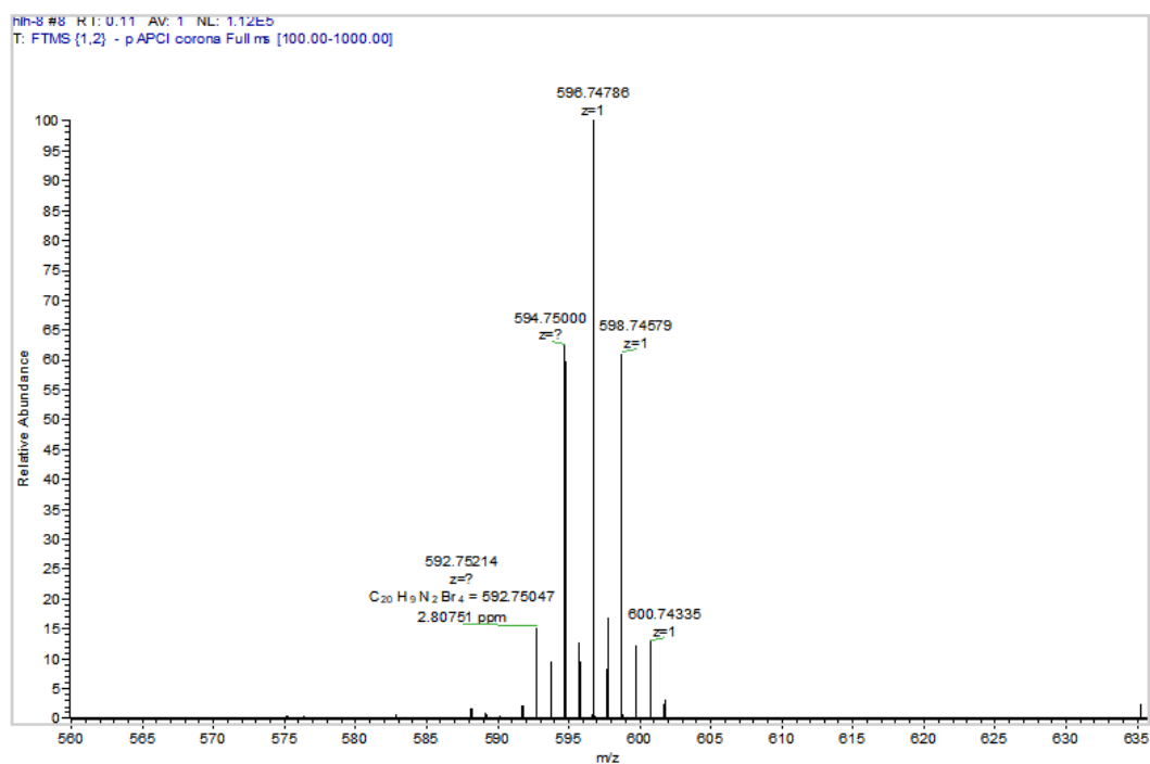
Figure S3. HRMS(APCI) spectrum of the compound of 5
