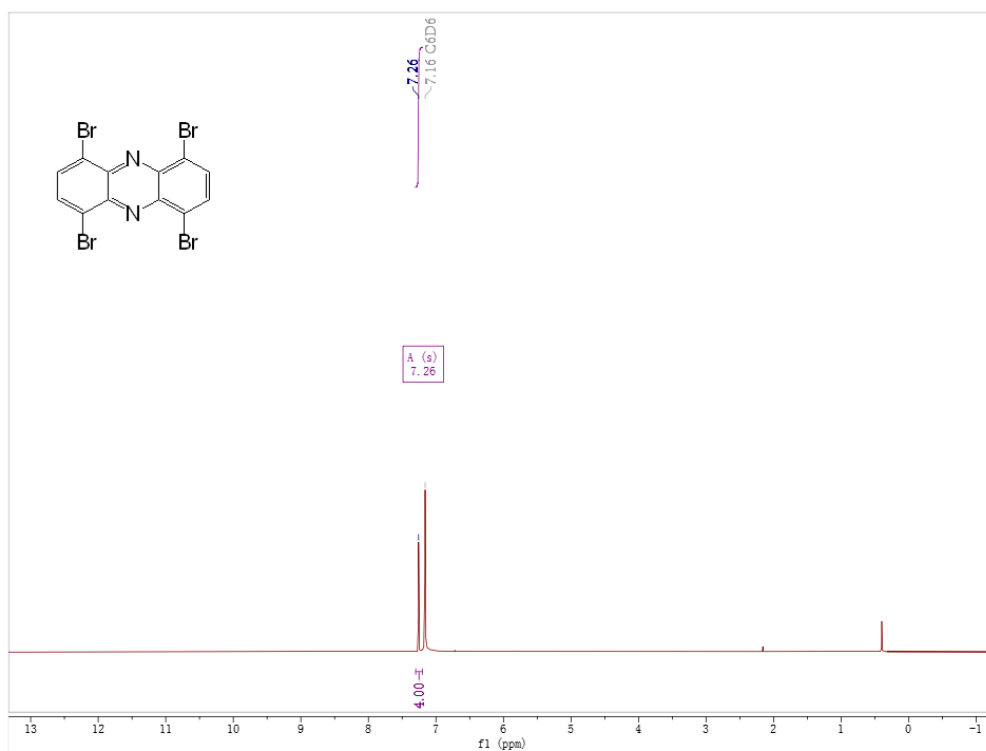
Figure S1. 1 H NMR spectrum of the compound 2
