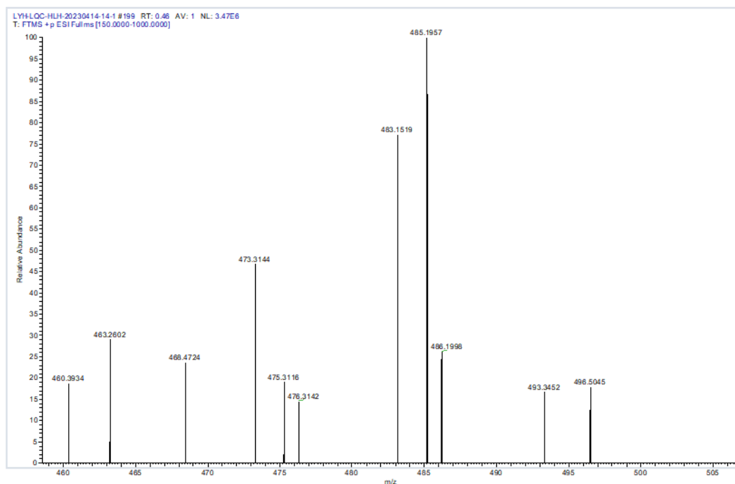
Figure S6. HRMS(ESI) spectrum of the compound of 3a
