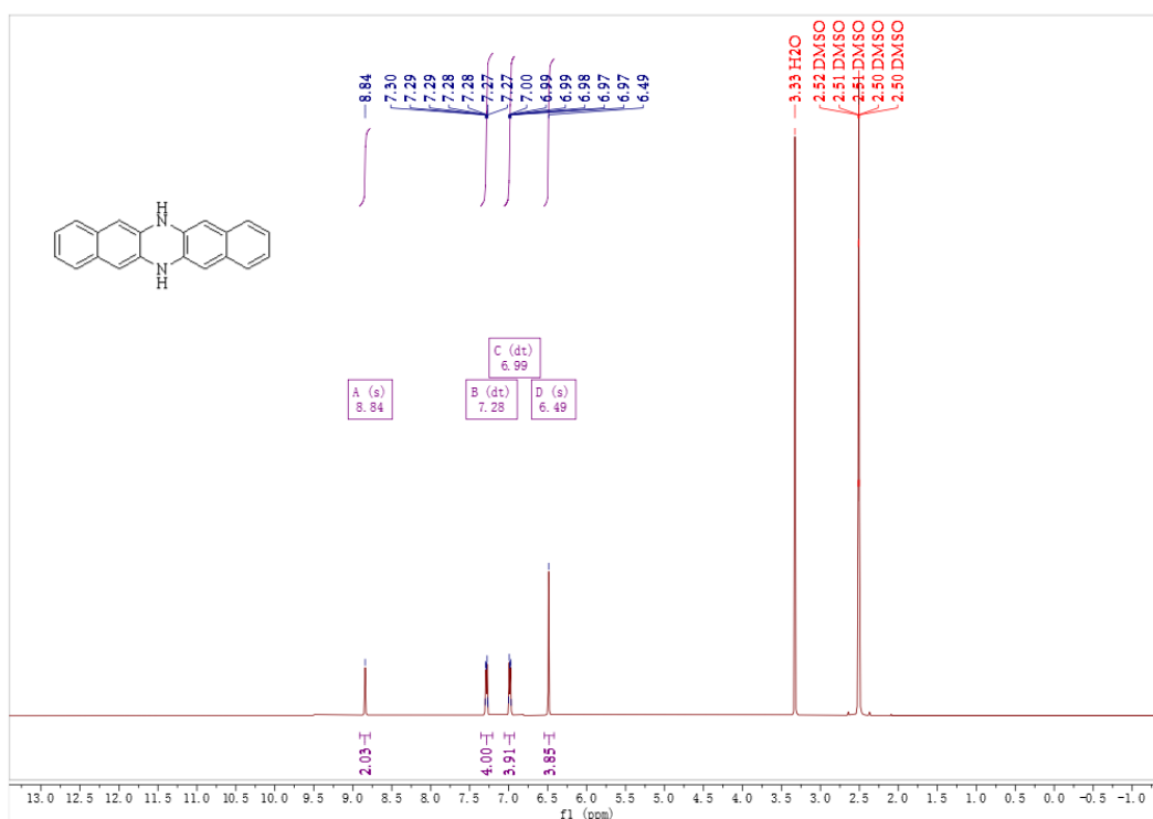
Figure S2. 1 H NMR spectrum of the compound of 4
