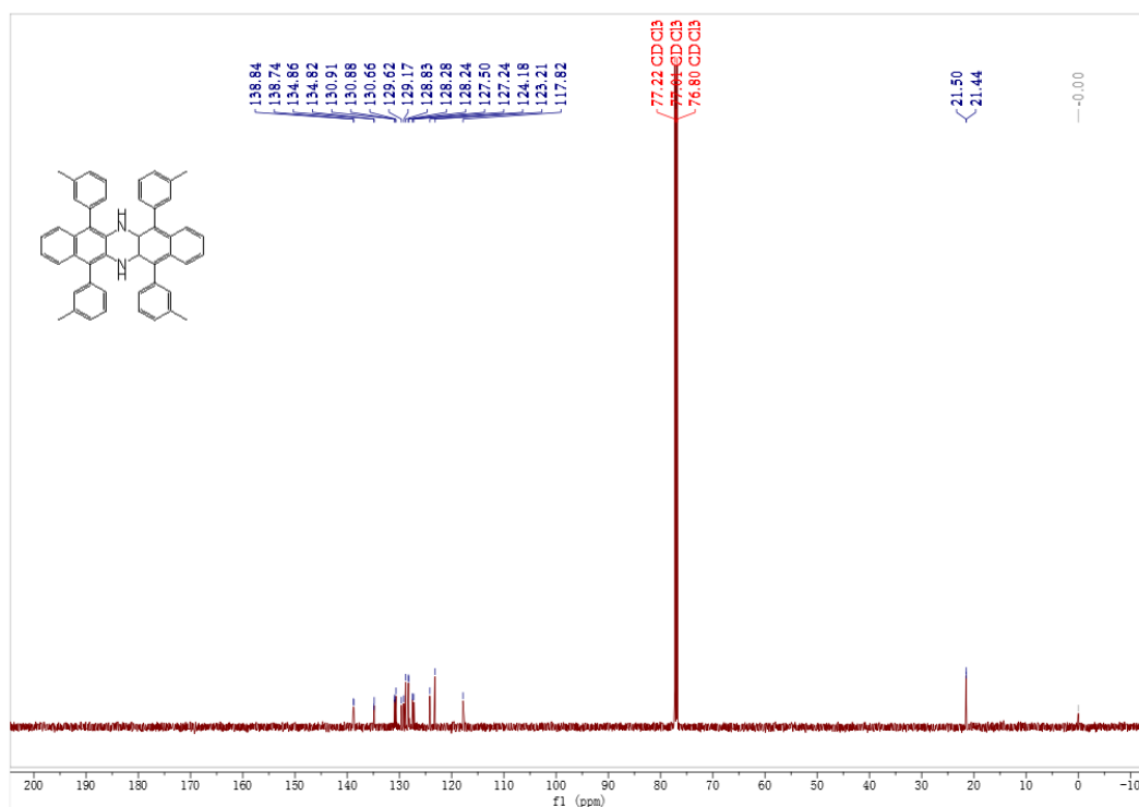
Figure S36. ^{13}\text{C} -NMR spectrum of the compound of 6c
