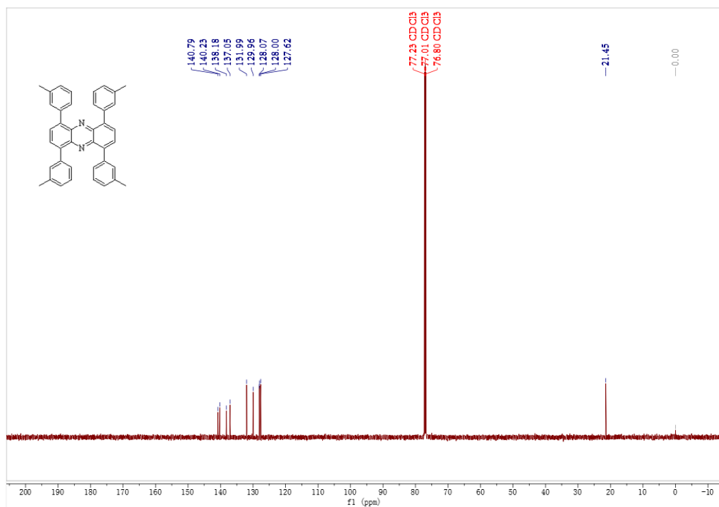
Figure S11. 13 C NMR spectrum of the compound of 3c
