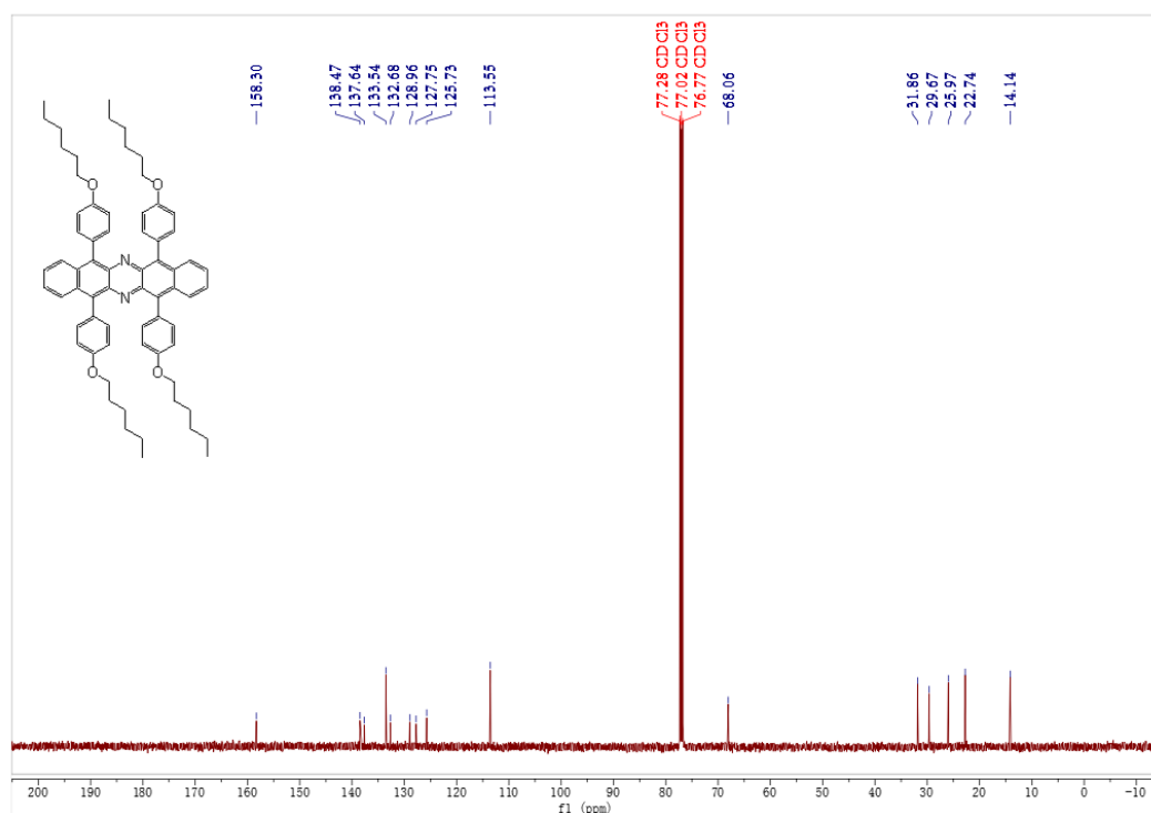
Figure S59. 13 C NMR spectrum of the compound of 7g
