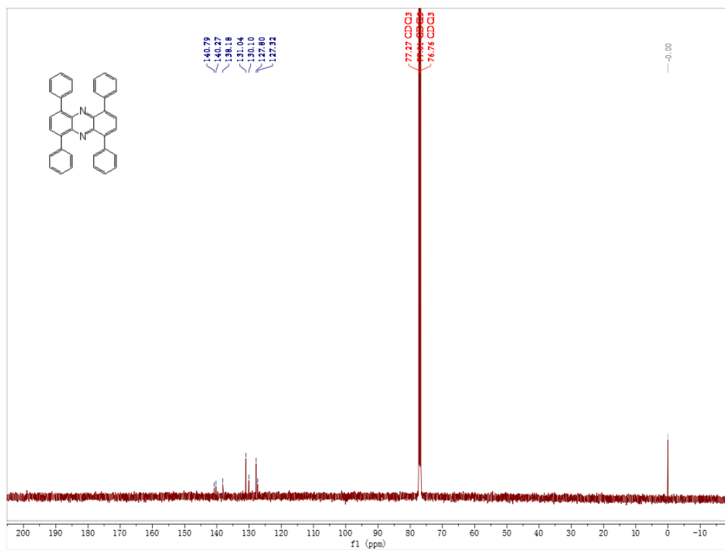
Figure S5. 13 C NMR spectrum of the compound of 3a
