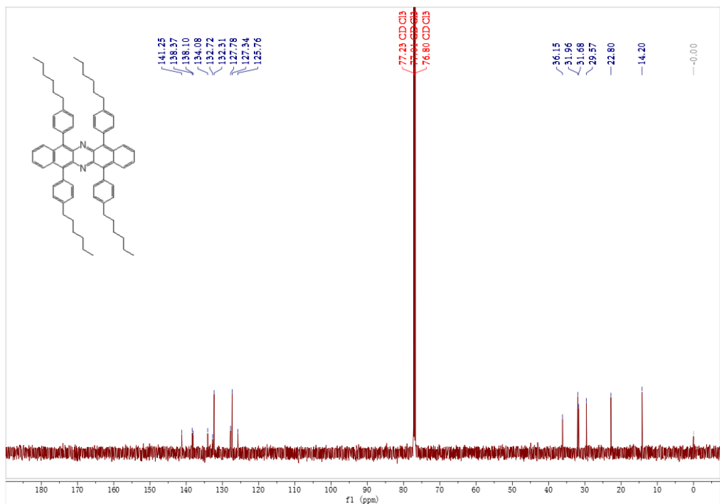
Figure S53. 13 C NMR spectrum of the compound of 7f
