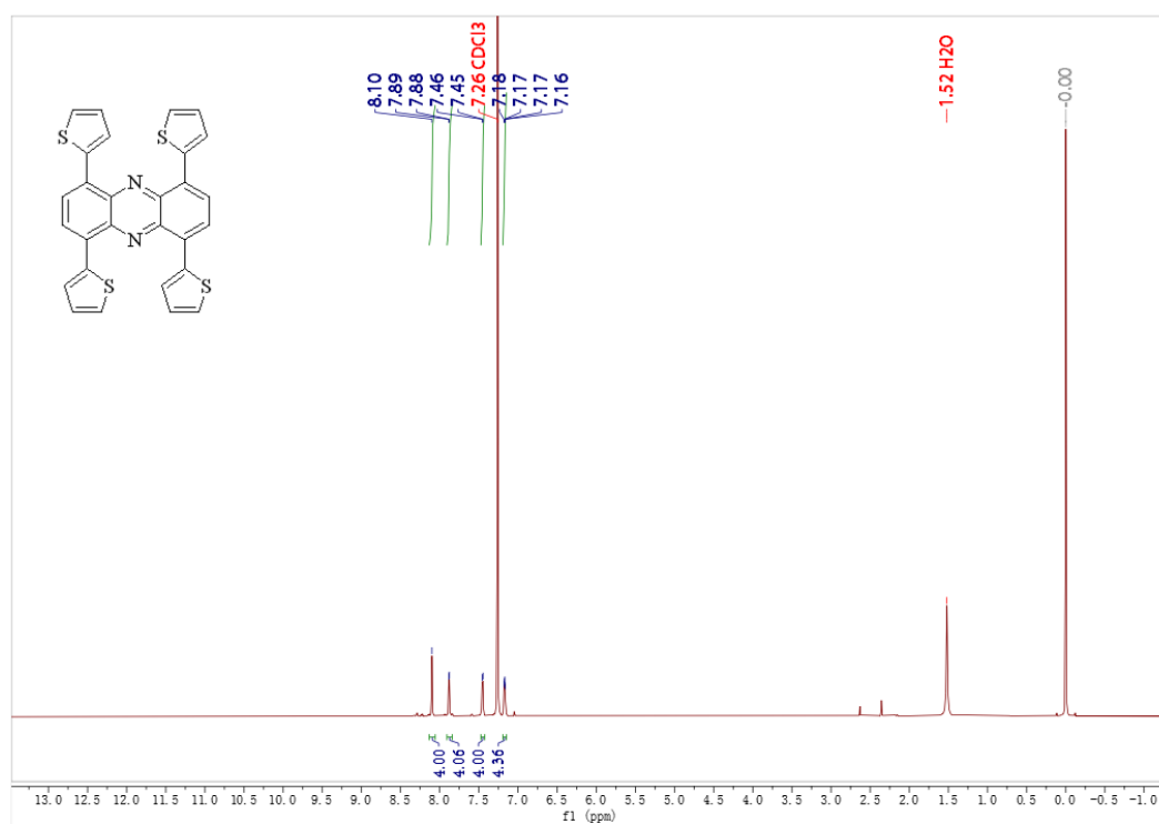
Figure S24. 1 H NMR spectrum of the compound of 3h
