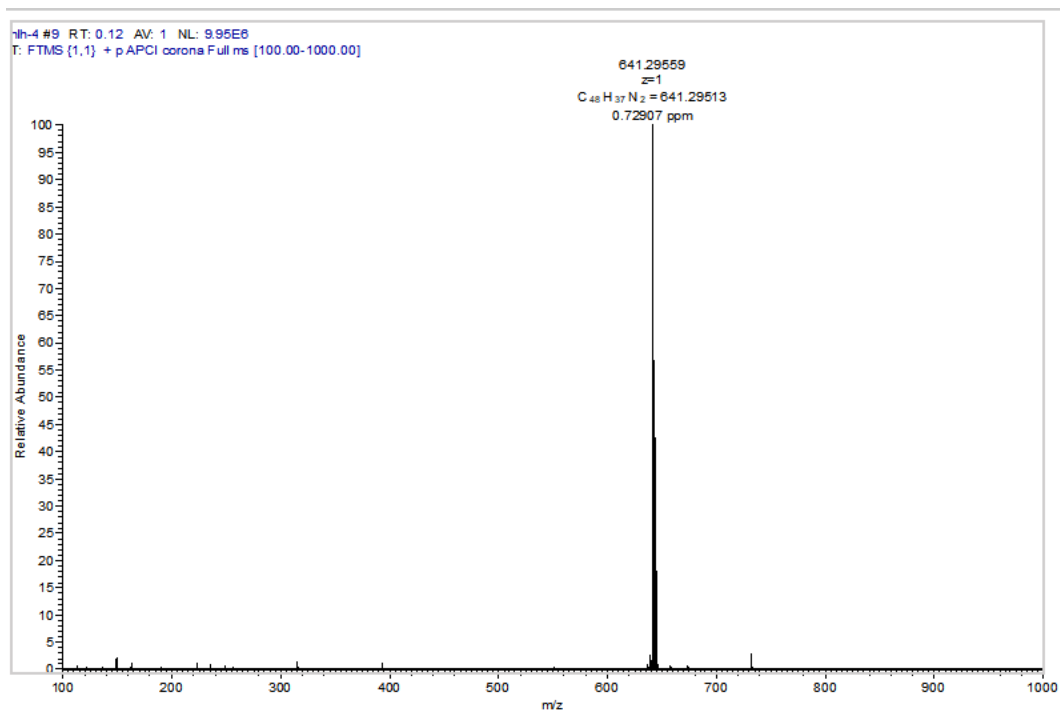
Figure S42. HRMS(APCI) spectrum of the compound of 7d
