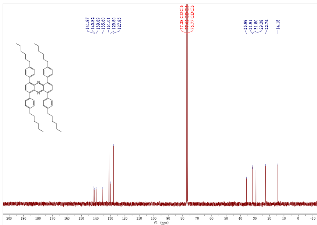
Figure S20. ^{13}\text{C} NMR spectrum of the compound of 3f
