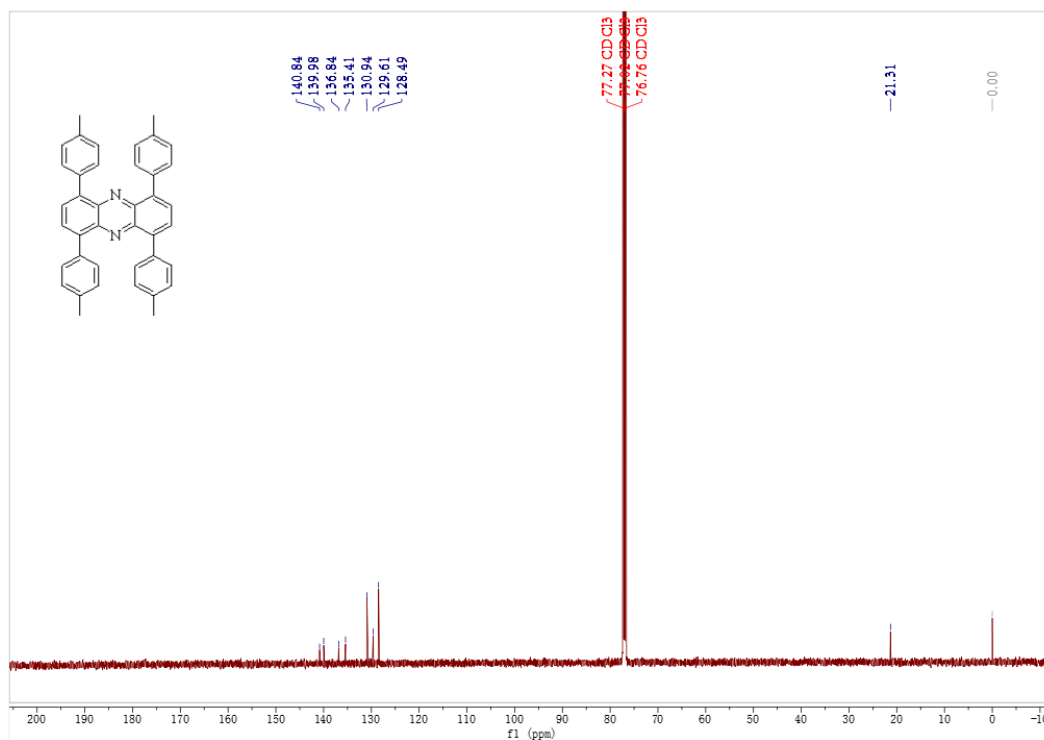
Figure S14. 13 C NMR spectrum of the compound of 3d
