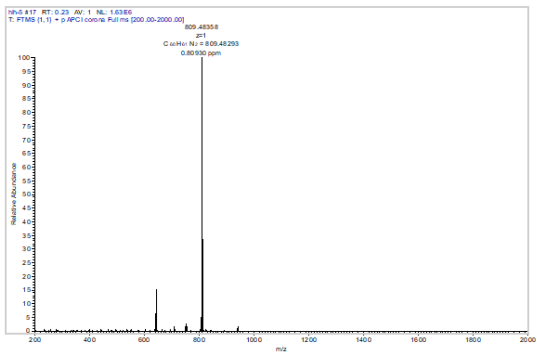
Figure S48. HRMS(APCI) spectrum of the compound of 7e
