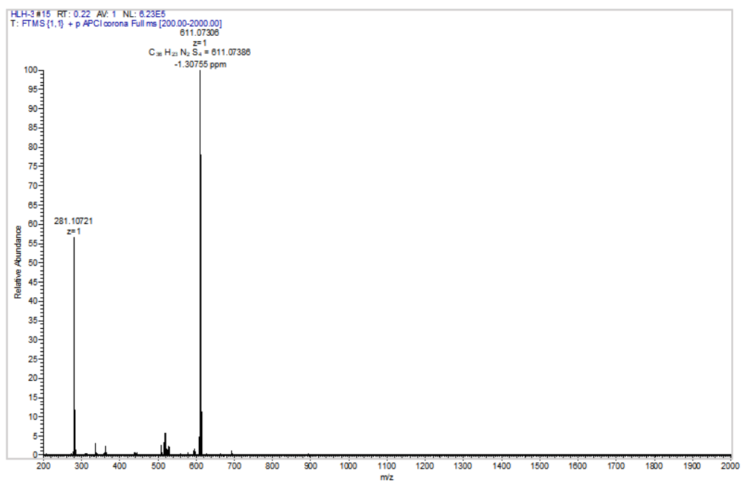
Figure S62. HRMS(APCI) spectrum of the compound of 6h
