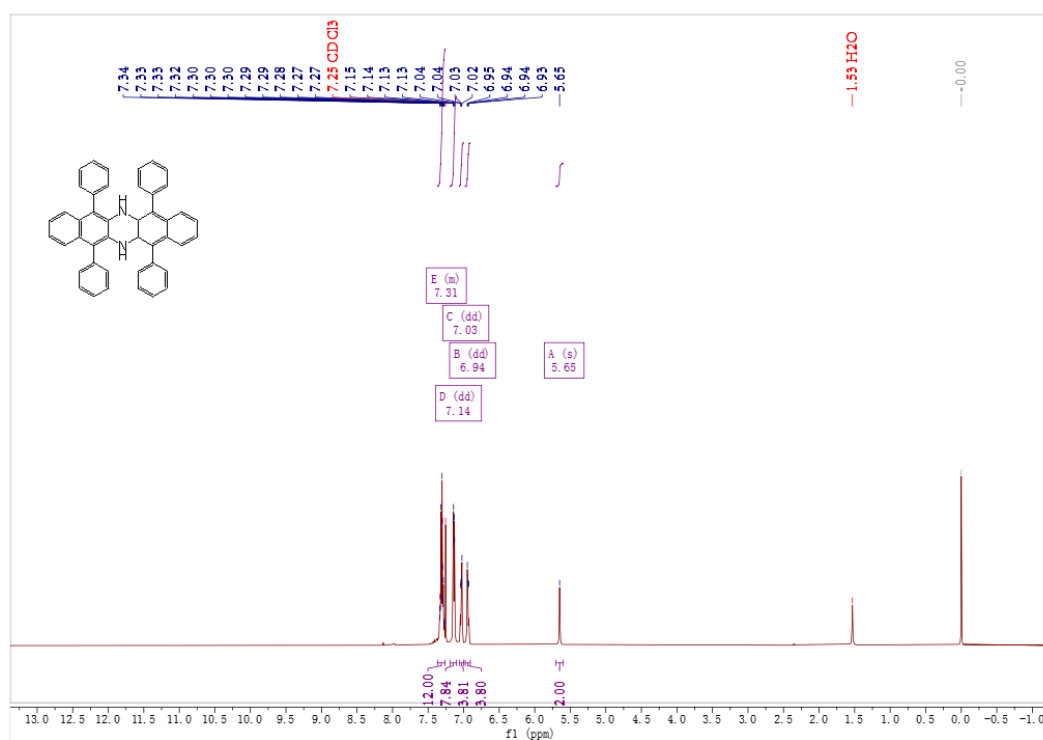
Figure S28. 1 H NMR spectrum of the compound of 6a
