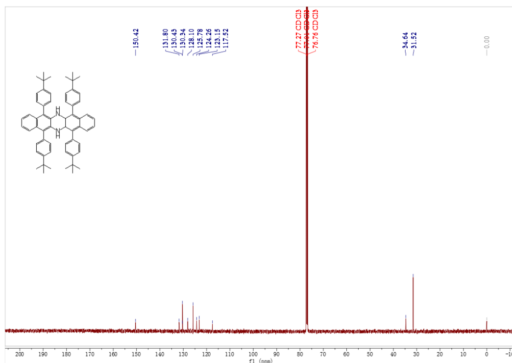
Figure S44. ^{13}\text{C} NMR spectrum of the compound of 6e
