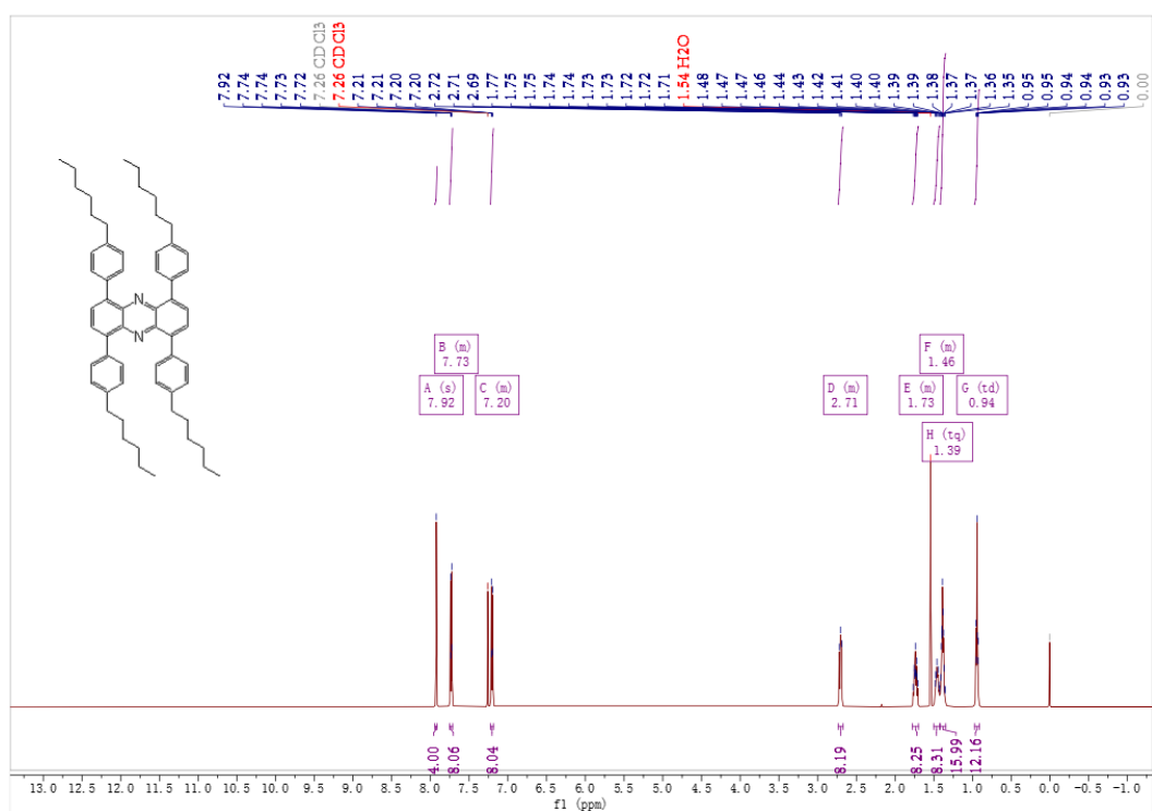
Figure S19. 1 H NMR spectrum of the compound of 3f
