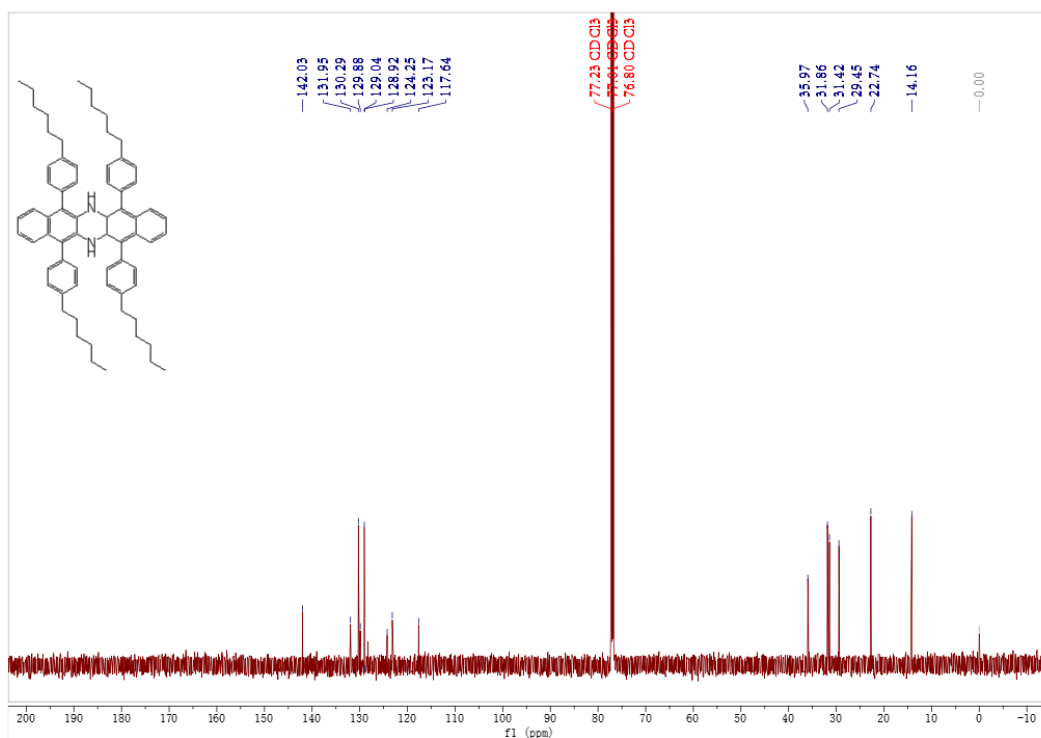
Figure S50. ^{13}\text{C} NMR spectrum of the compound of 6f
