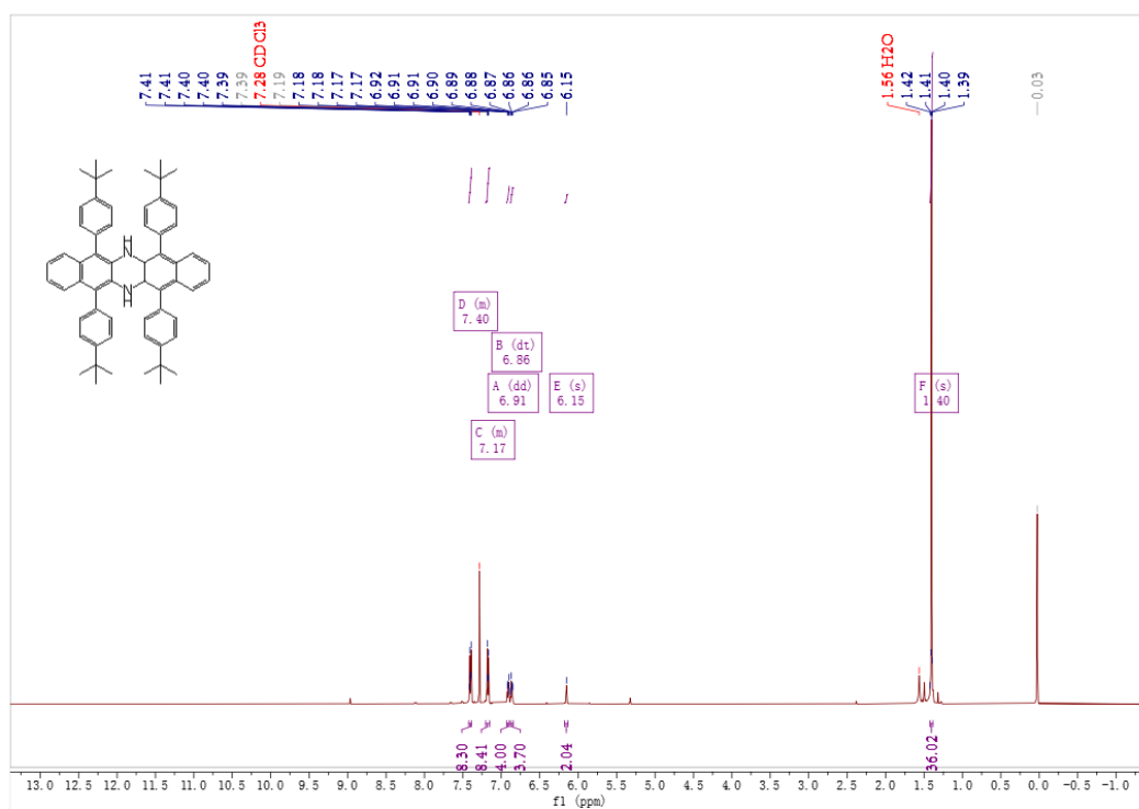
Figure S43. 1 H NMR spectrum of the compound of 6e
