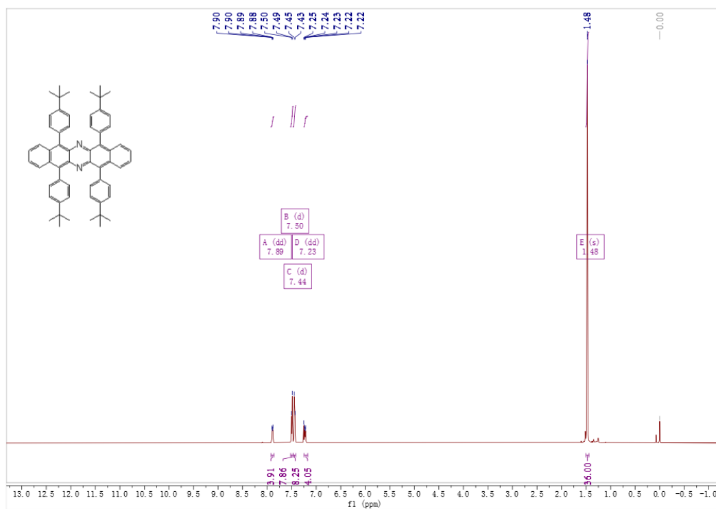
Figure S46. 1 H NMR spectrum of the compound of 7e
