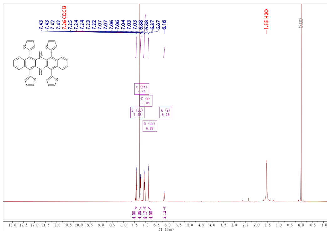
Figure S61. 1 H NMR spectrum of the compound of 6h
