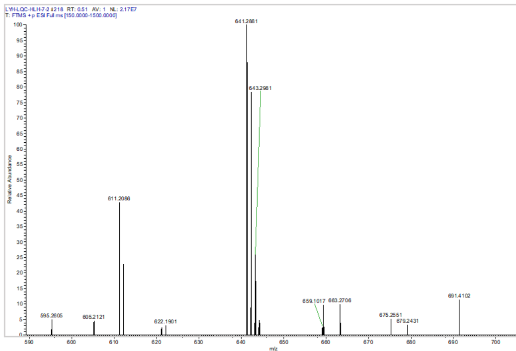
Figure S34. HRMS(ESI) spectrum of the compound of 7b
