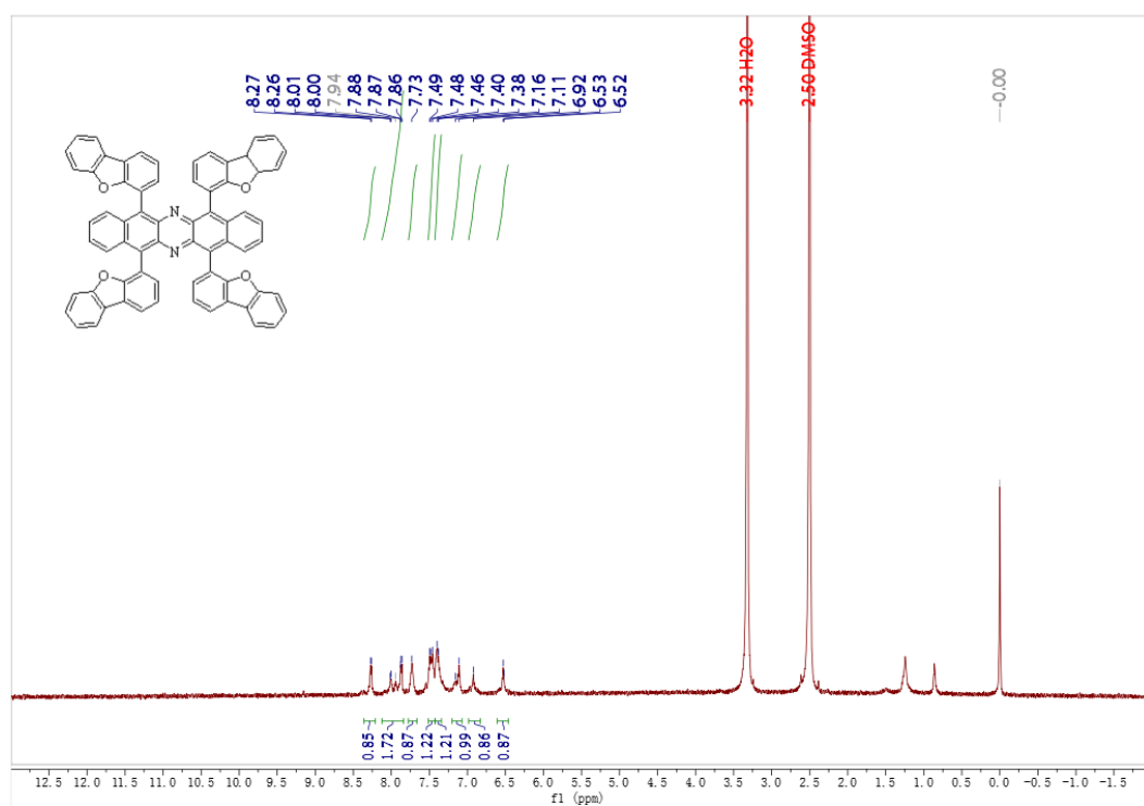
Figure S67. ^1\text{H} NMR spectrum of the compound of 7i
