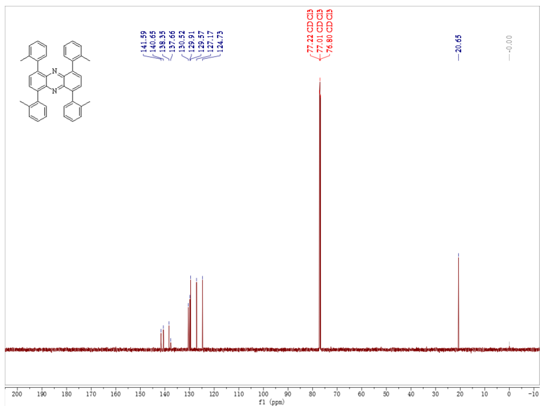
Figure S8. 13 C NMR spectrum of the compound of 3b
