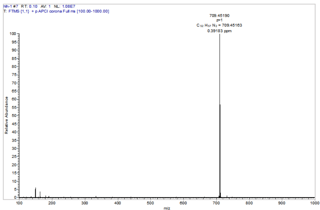
Figure S18. HRMS(APCI) spectrum of the compound of 3e
