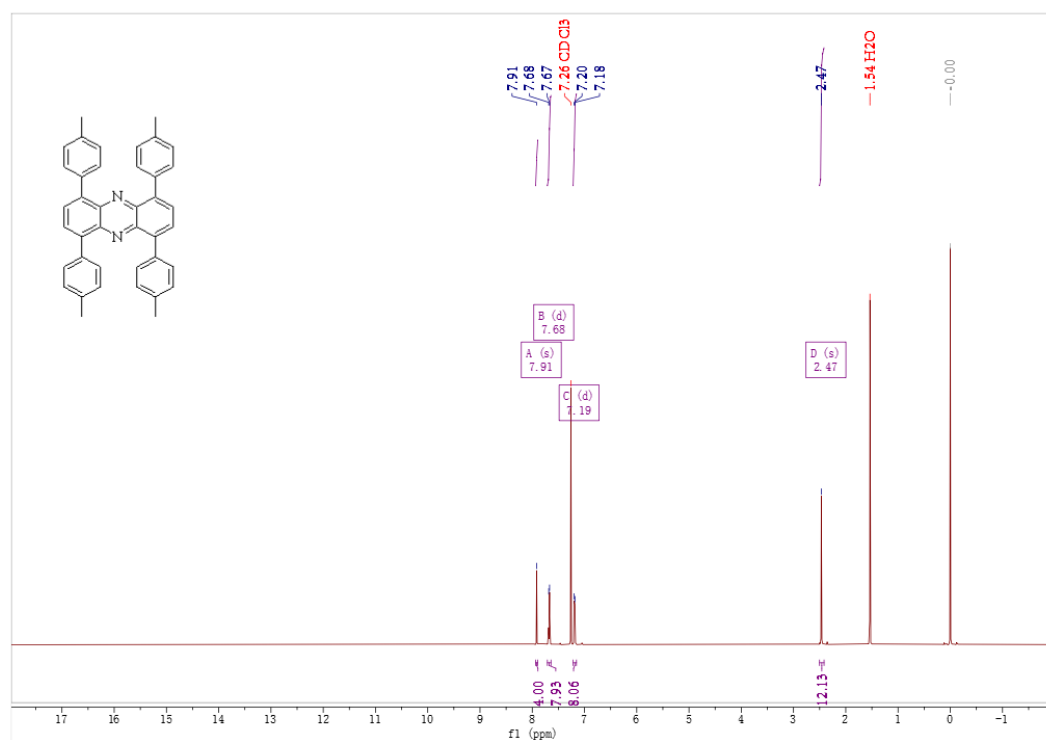
Figure S13. ^1\text{H} NMR spectrum of the compound of 3d
