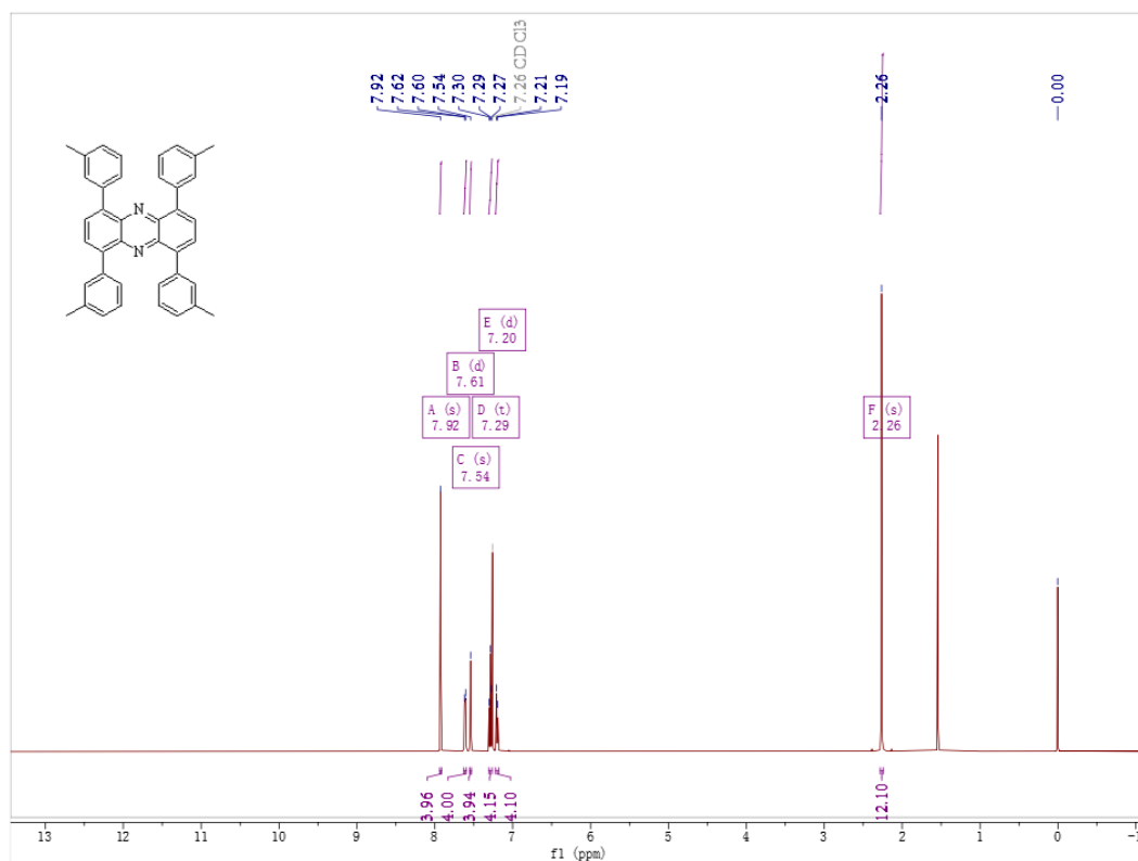
Figure S10. 1 H NMR spectrum of the compound of 3c
