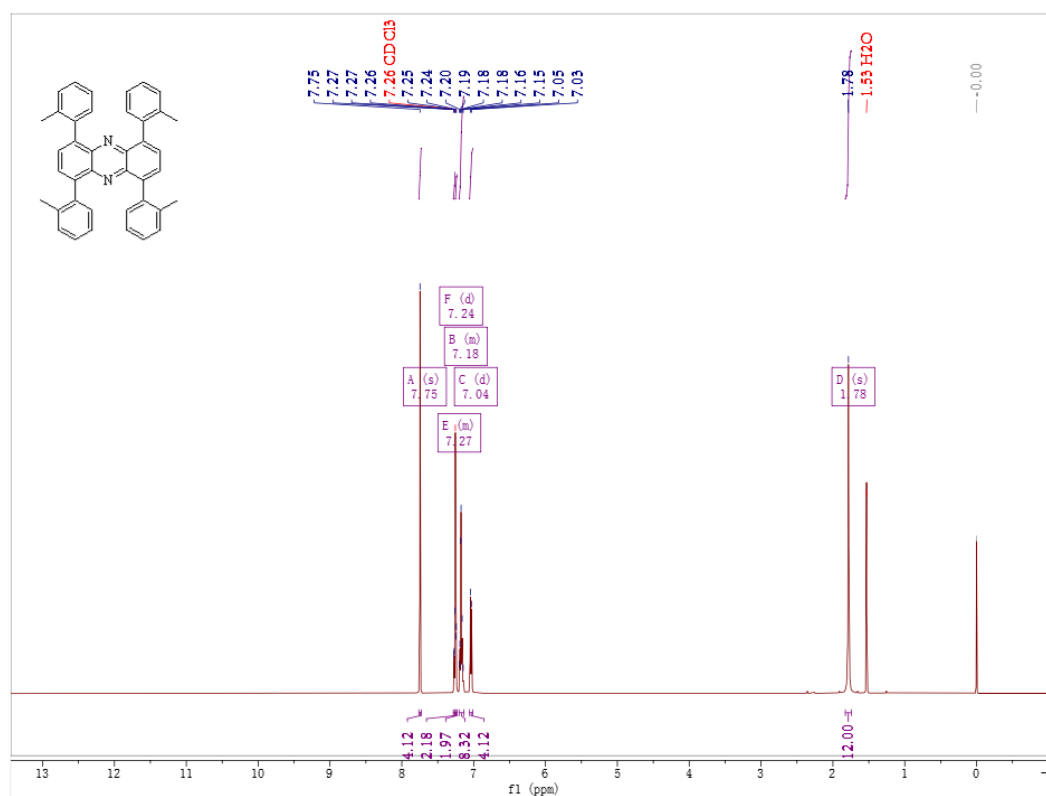
Figure S7. ^1\text{H} NMR spectrum of the compound of 3b
