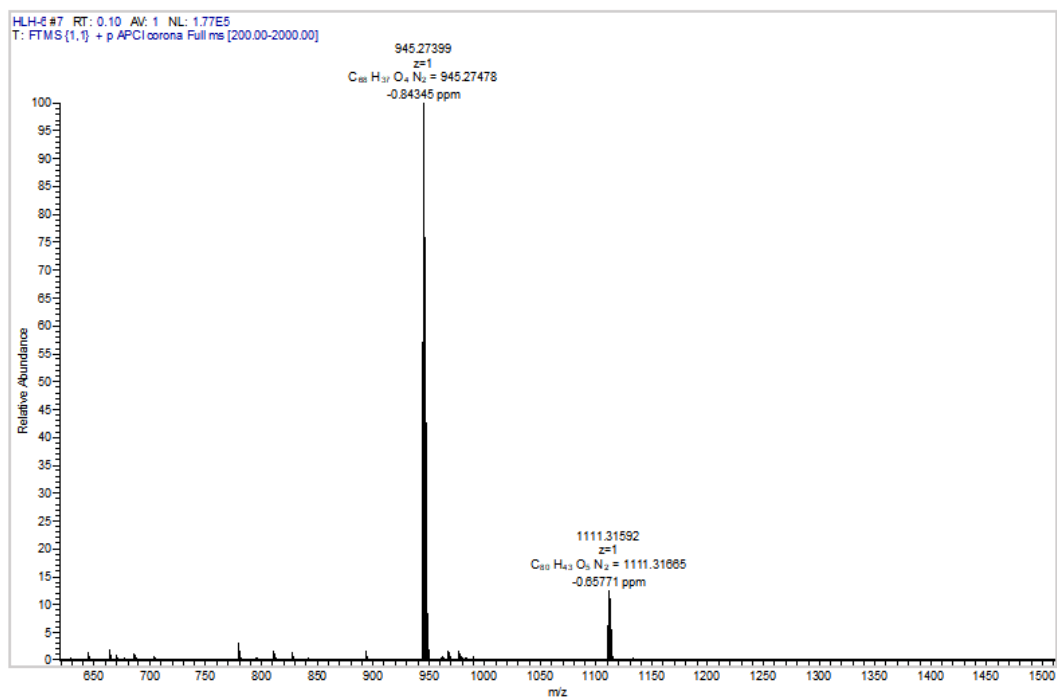
Figure S68. HRMS (APCI) spectrum of the compound of 7i
