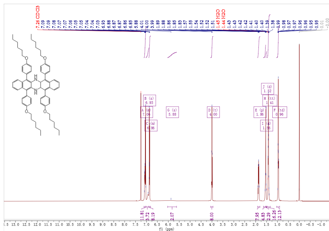
Figure S55. ^1\text{H} NMR spectrum of the compound of 6g
