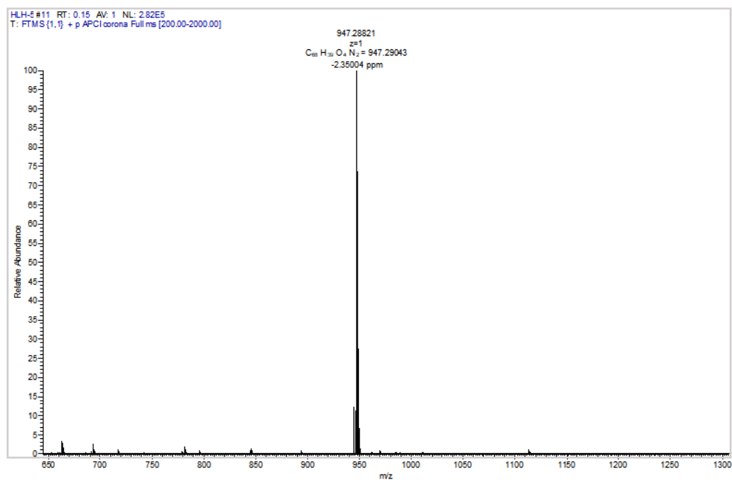
Figure S66. HRMS(APCI) spectrum of the compound of 6i
