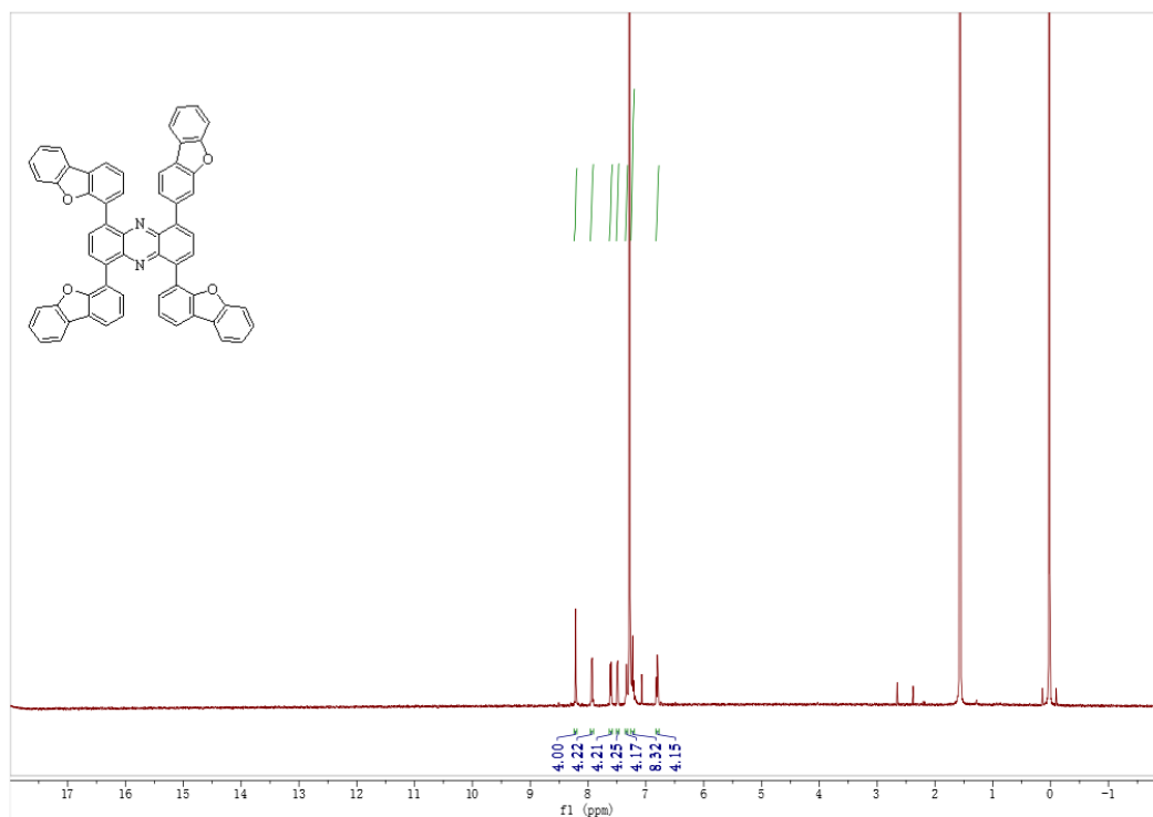
Figure S26. ^1\text{H} NMR spectrum of the compound of 3i
