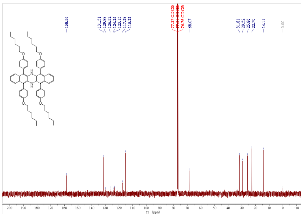
Figure S56. ^{13}\text{C} NMR spectrum of the compound of 6g
