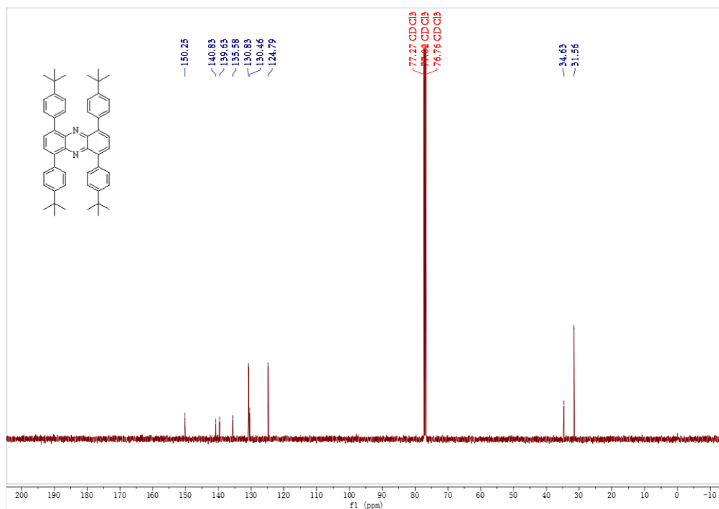
Figure S17. 13 C NMR spectrum of the compound of 3e
