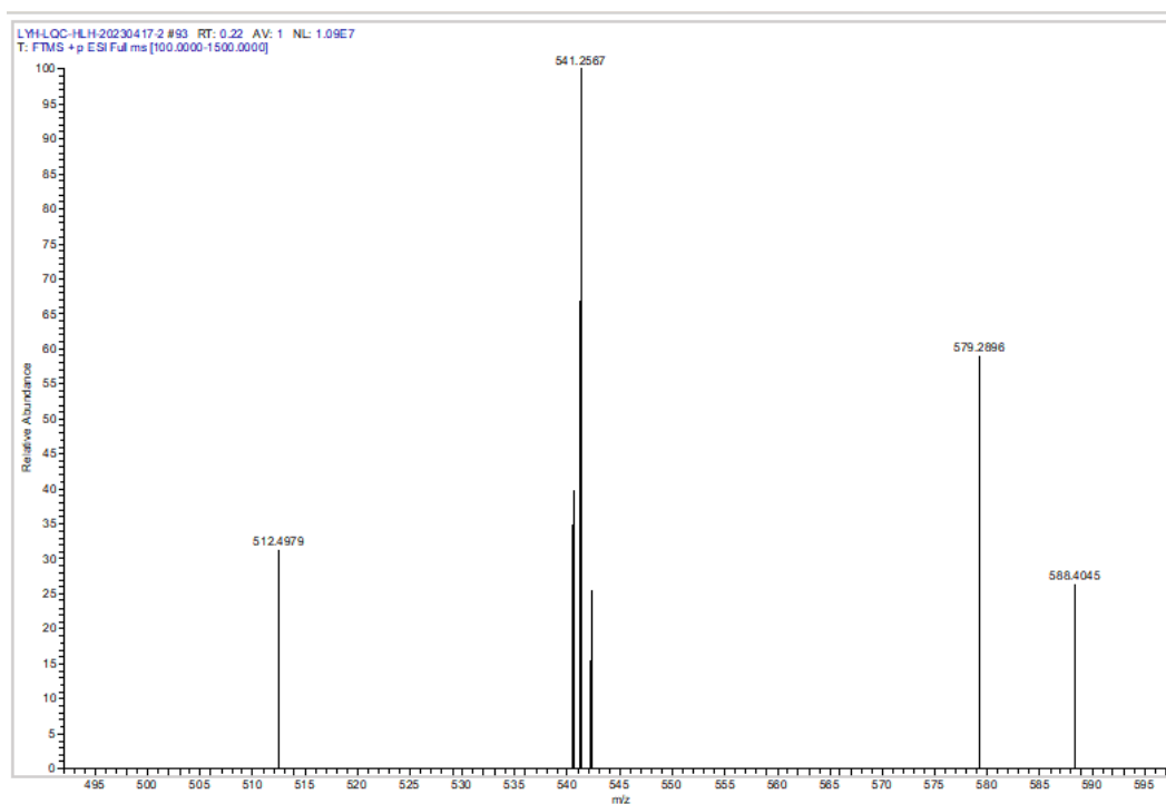
Figure S15. HRMS(ESI) spectrum of the compound of 3d
