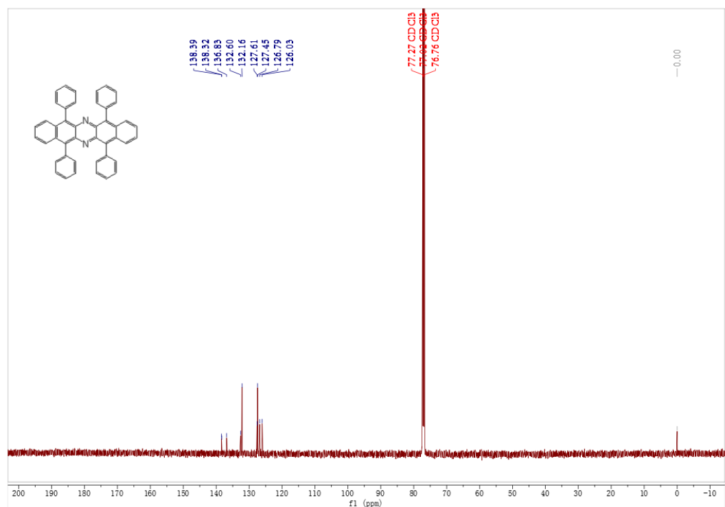
Figure S31. 13 C-NMR spectrum of the compound of 7a
