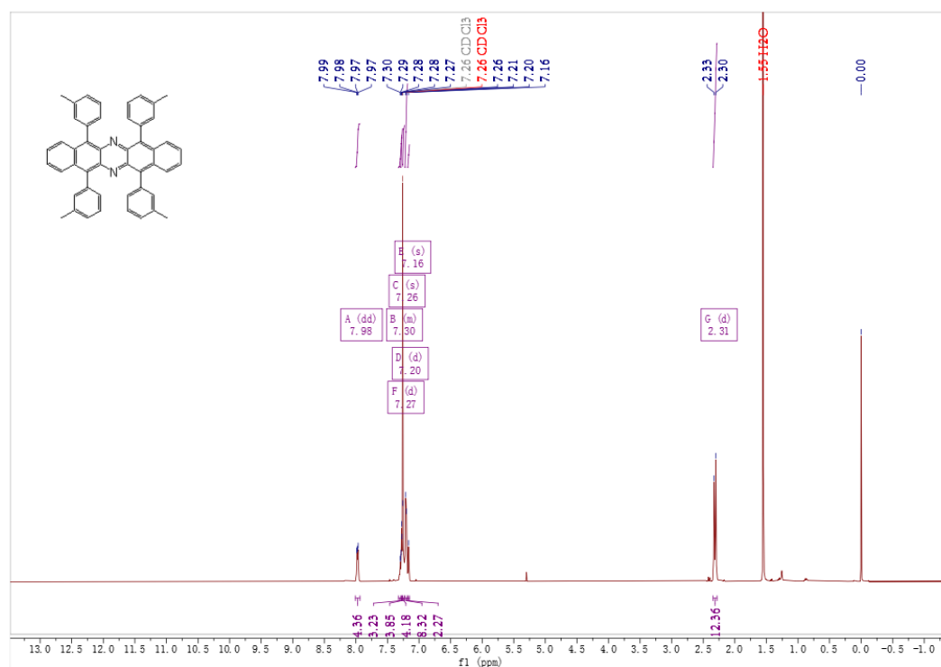
Figure S37. ^1\text{H} NMR spectrum of the compound of 7c
