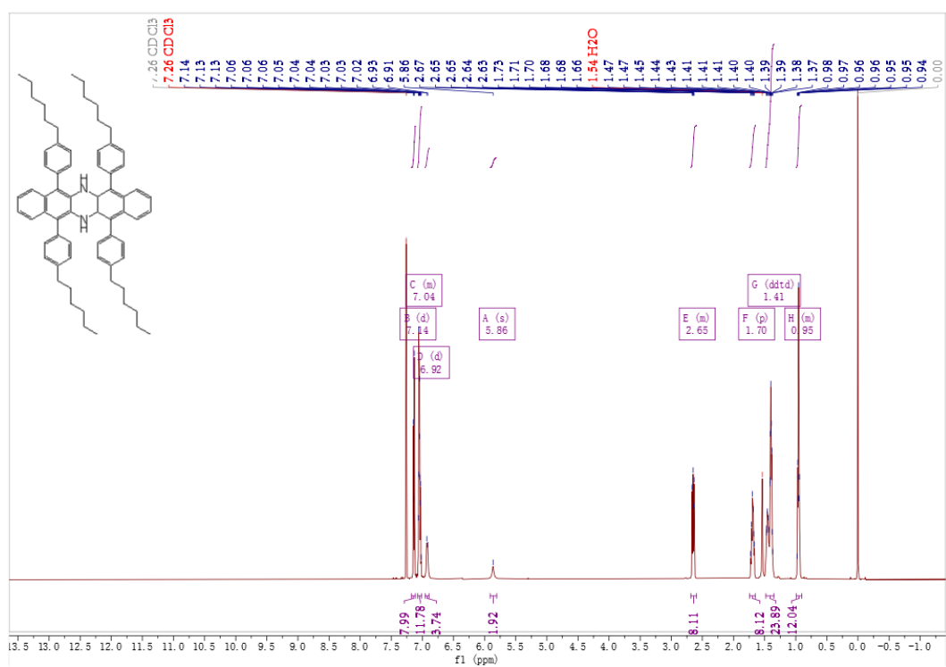
Figure S49. 1 H NMR spectrum of the compound of 6f
