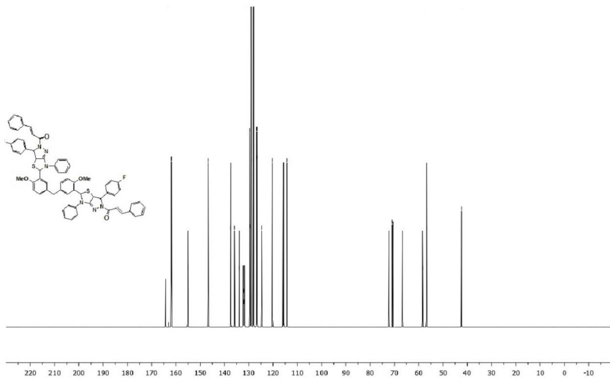
13 C NMR spectrum of compound 5a in CDCl 3 , 75 MHz
