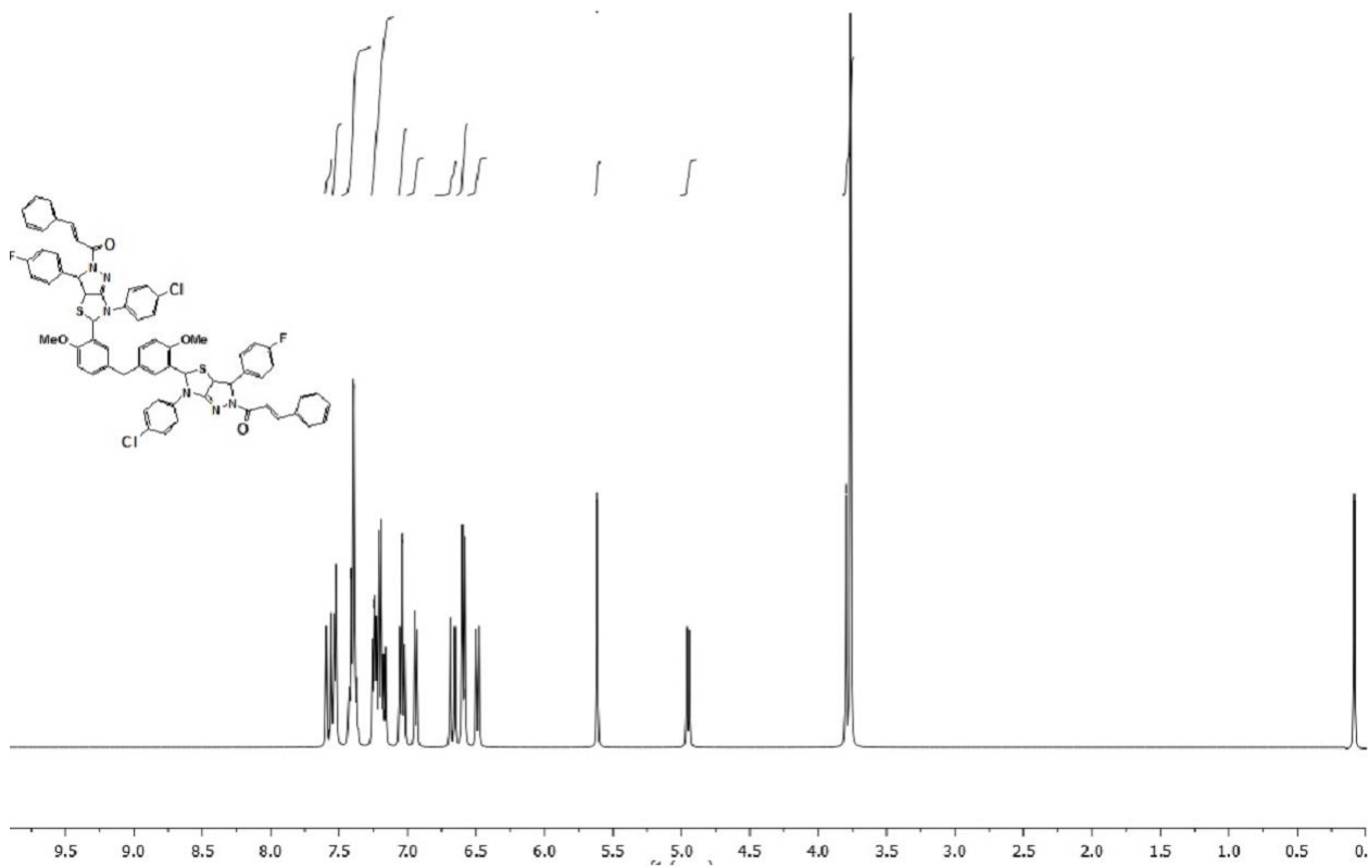
13 C NMR spectrum of compound 5a in CDCl 3 , 75 MHz
