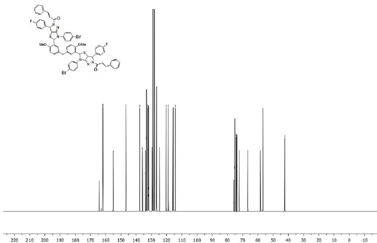
^{13}\text{C} NMR spectrum of compound 5c in \text{CDCl}_3 , 75 MHz
