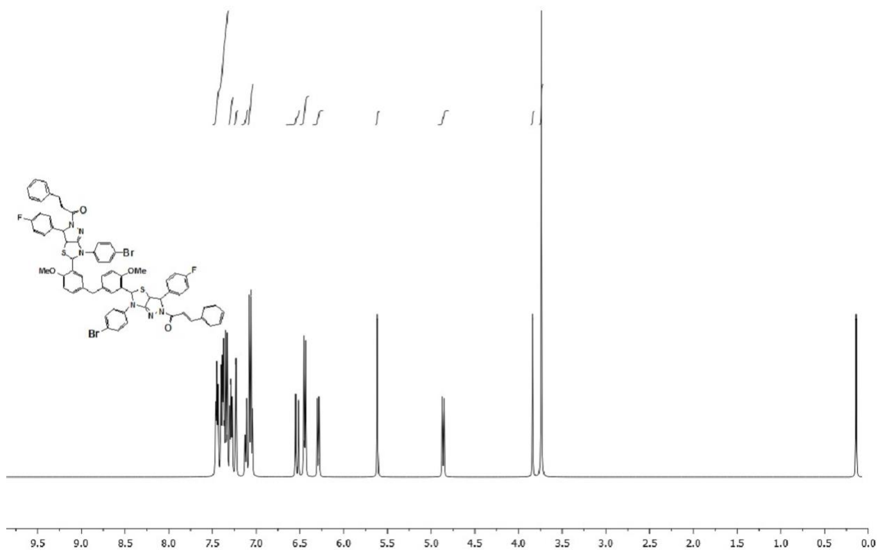
^1\text{H} NMR spectrum of compound 5c in \text{CDCl}_3 , 300 MHz
