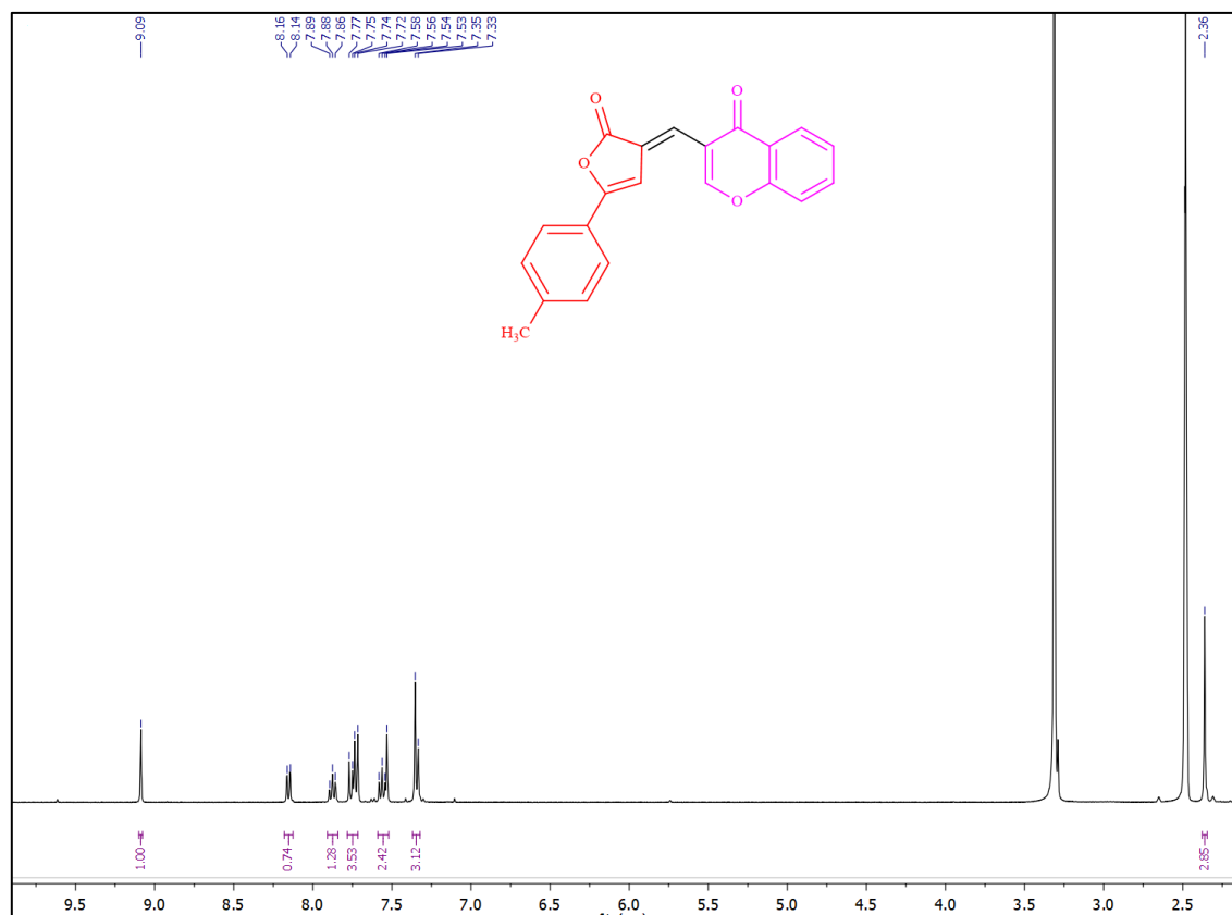
Fig. S2. ^1\text{H} & ^{13}\text{C} of 3b
