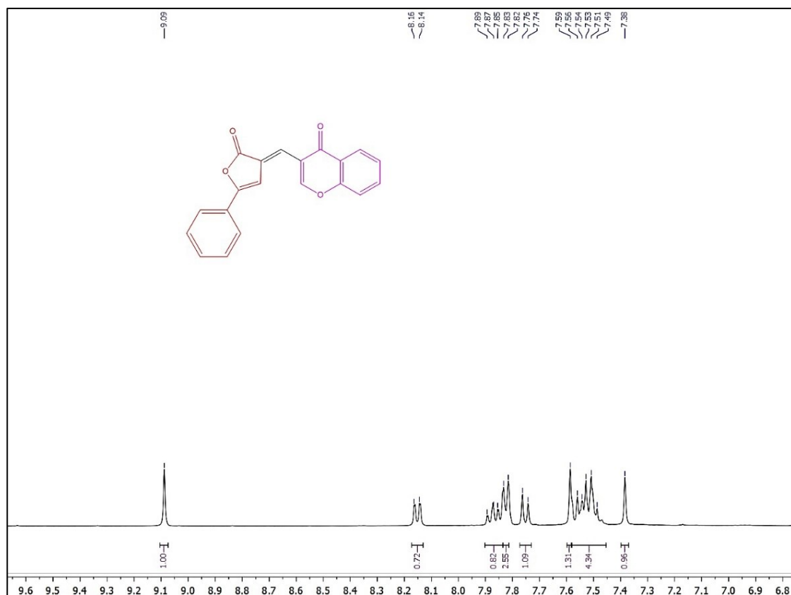
Fig. S1. ^1\text{H} & ^{13}\text{C} , NOESY of 3a
