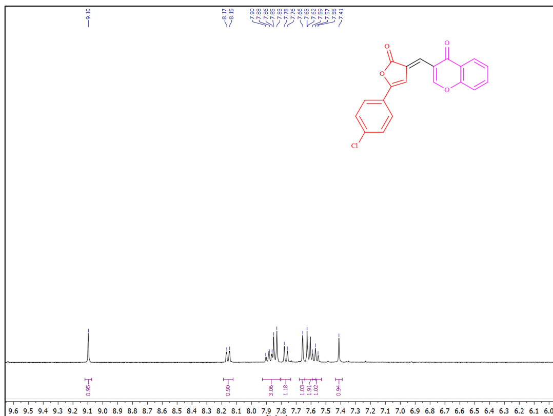
Fig. S3. ^1\text{H} & ^{13}\text{C} of 3c
