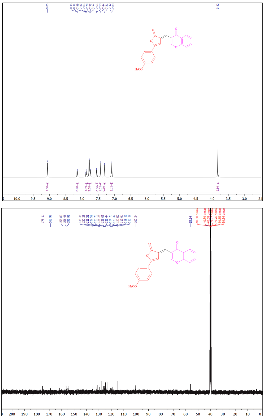
Fig. S6. ^1\text{H} & ^{13}\text{C} of 3f
