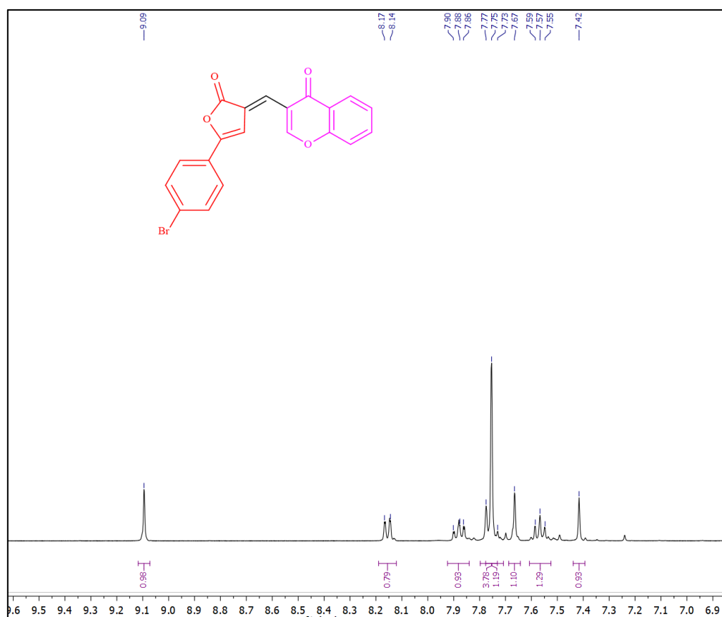
Fig. S4. ^1\text{H} & ^{13}\text{C} of 3d
