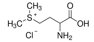
S-methyl methionine sulfonium chloride (MMSC)
