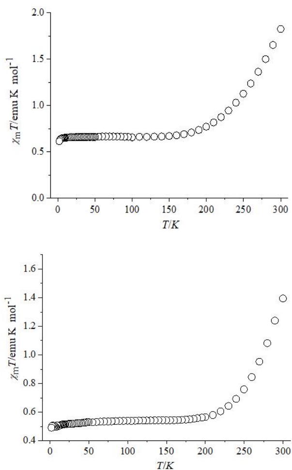
Figure S1. Temperature dependences of \chi_m T of 4 (top) and 5 (bottom).
