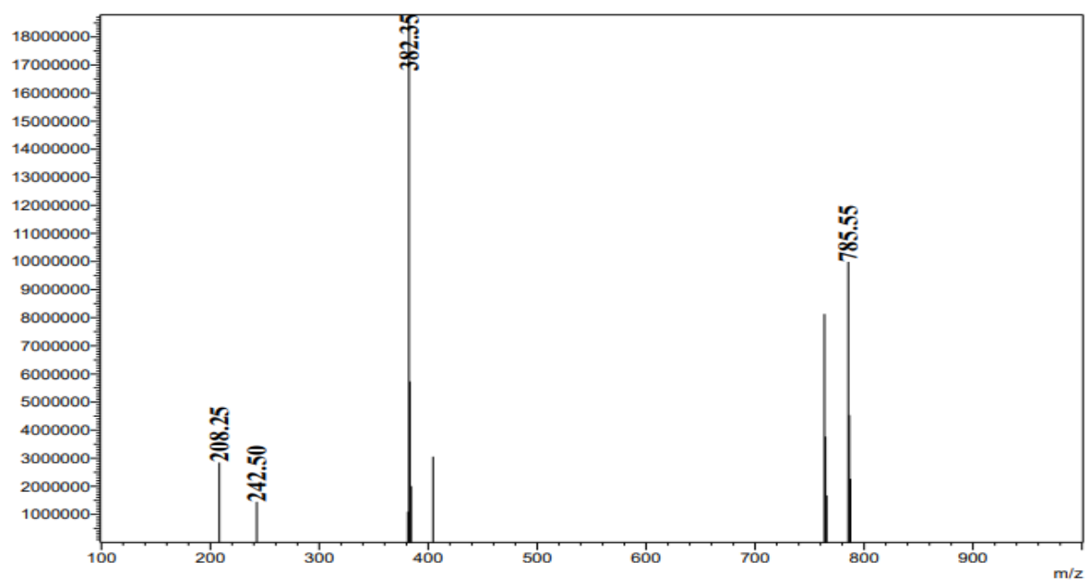
Figure S28. LC/MS spectrum of compound 3g
