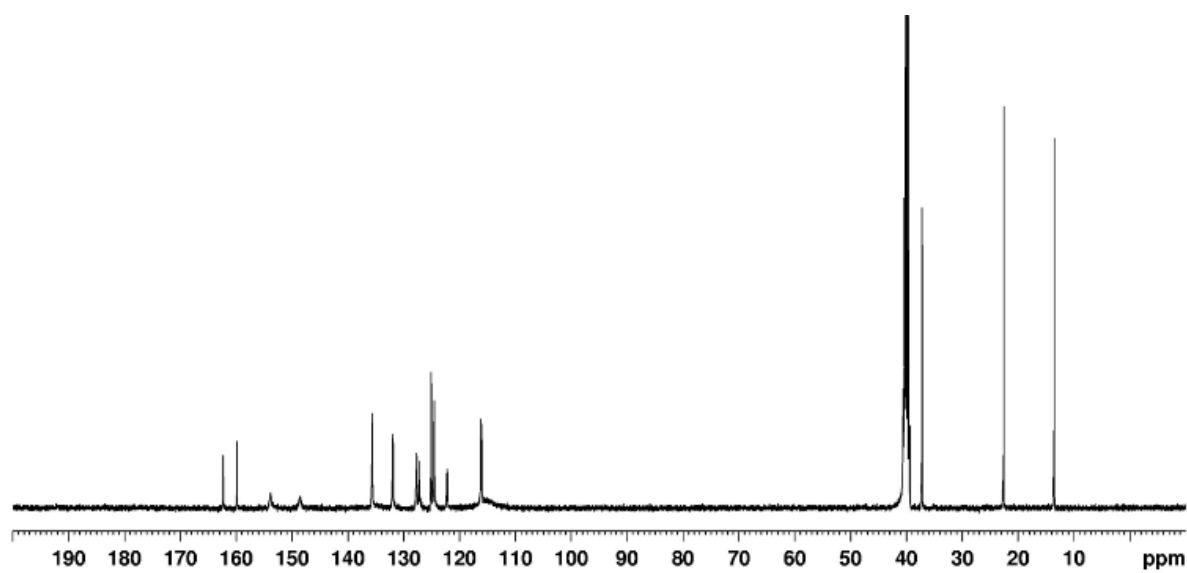
Figure S7. ^{13}\text{C} -NMR spectrum of compound 3b
