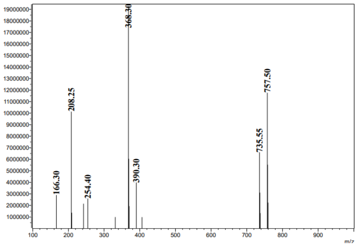
Figure S20. LC/MS spectrum of compound 3e
