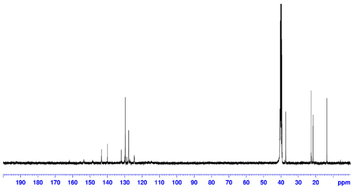
Figure S19. ^{13}\text{C} -NMR spectrum of compound 3e
