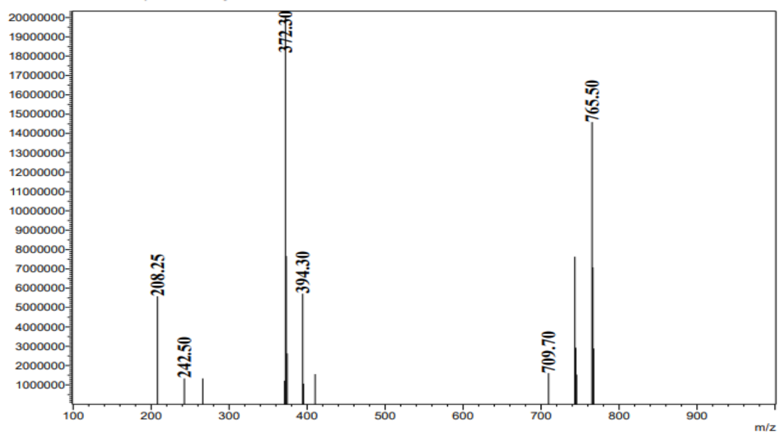
Figure S12. LC/MS spectrum of compound 3c
