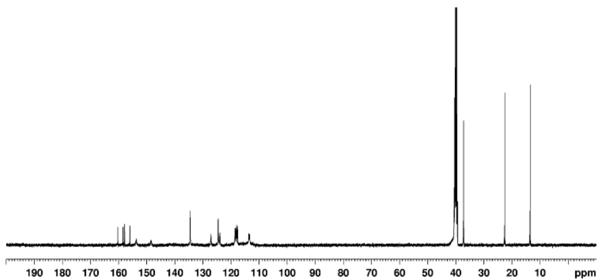
Figure S15. ^{13}\text{C} -NMR spectrum of compound 3d
