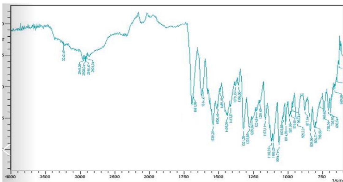
Figure S33. IR spectrum of compound 3i
