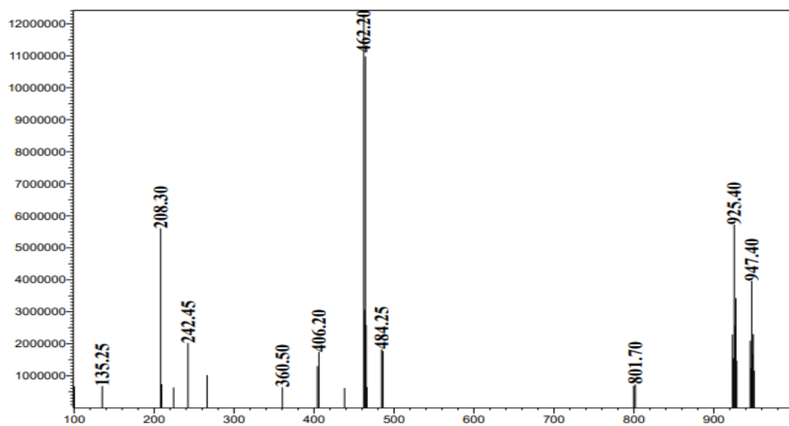
Figure S32. LC/MS spectrum of compound 3h
