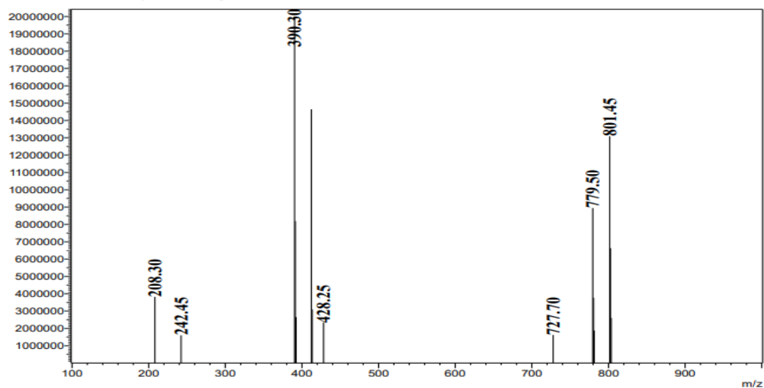
Figure S16. LC/MS spectrum of compound 3d
