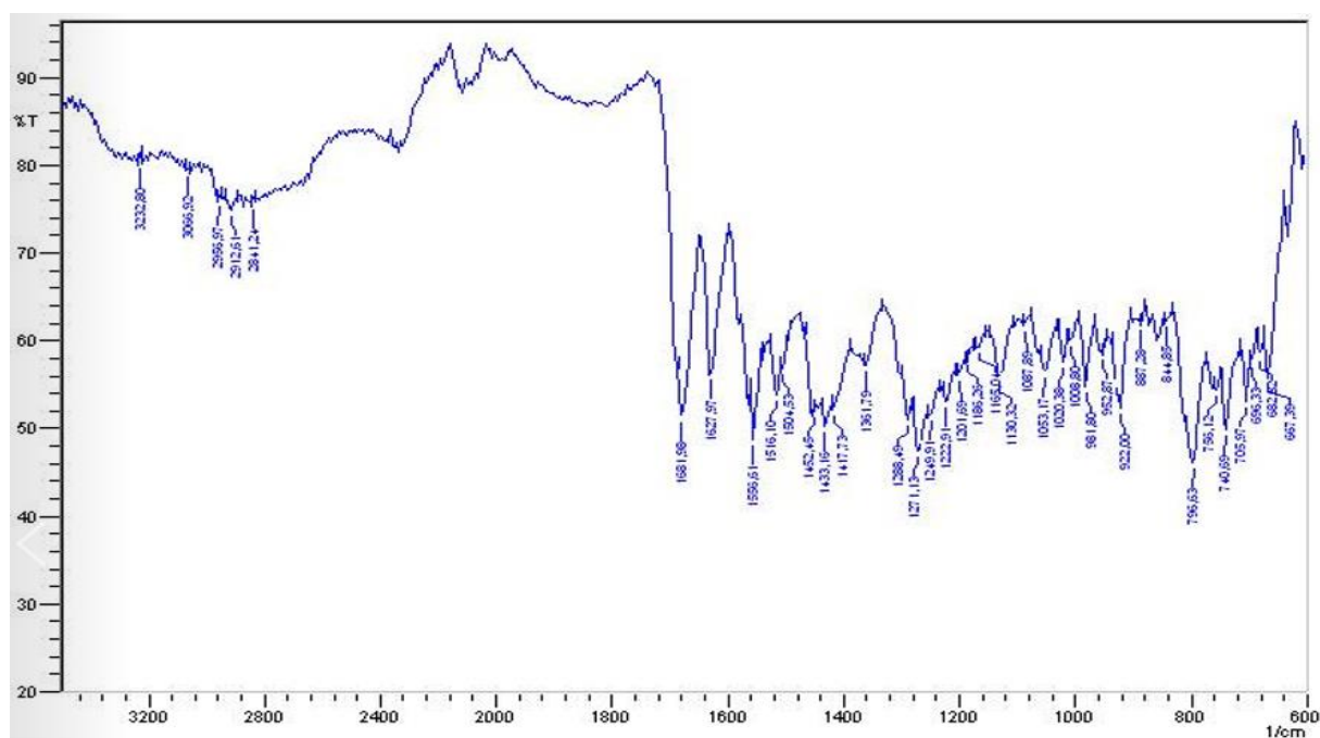
Figure S25. IR spectrum of compound 3g
