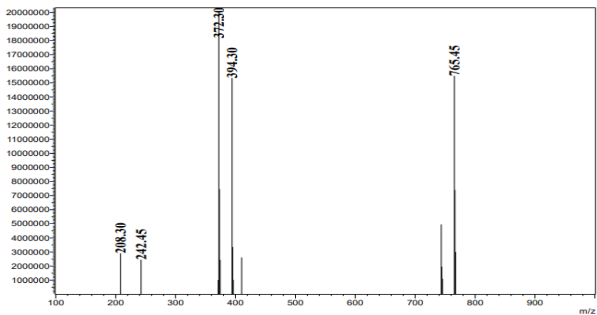
Figure S8. LC/MS spectrum of compound 3b
