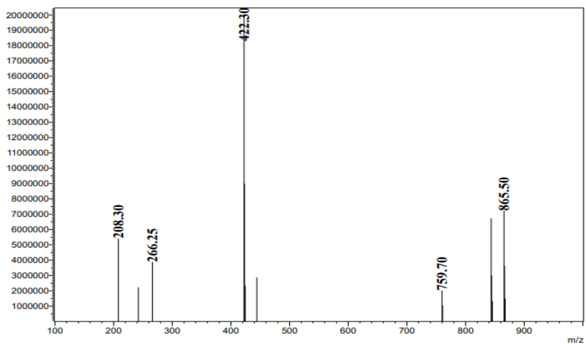
Figure S36. LC/MS spectrum of compound 3i
