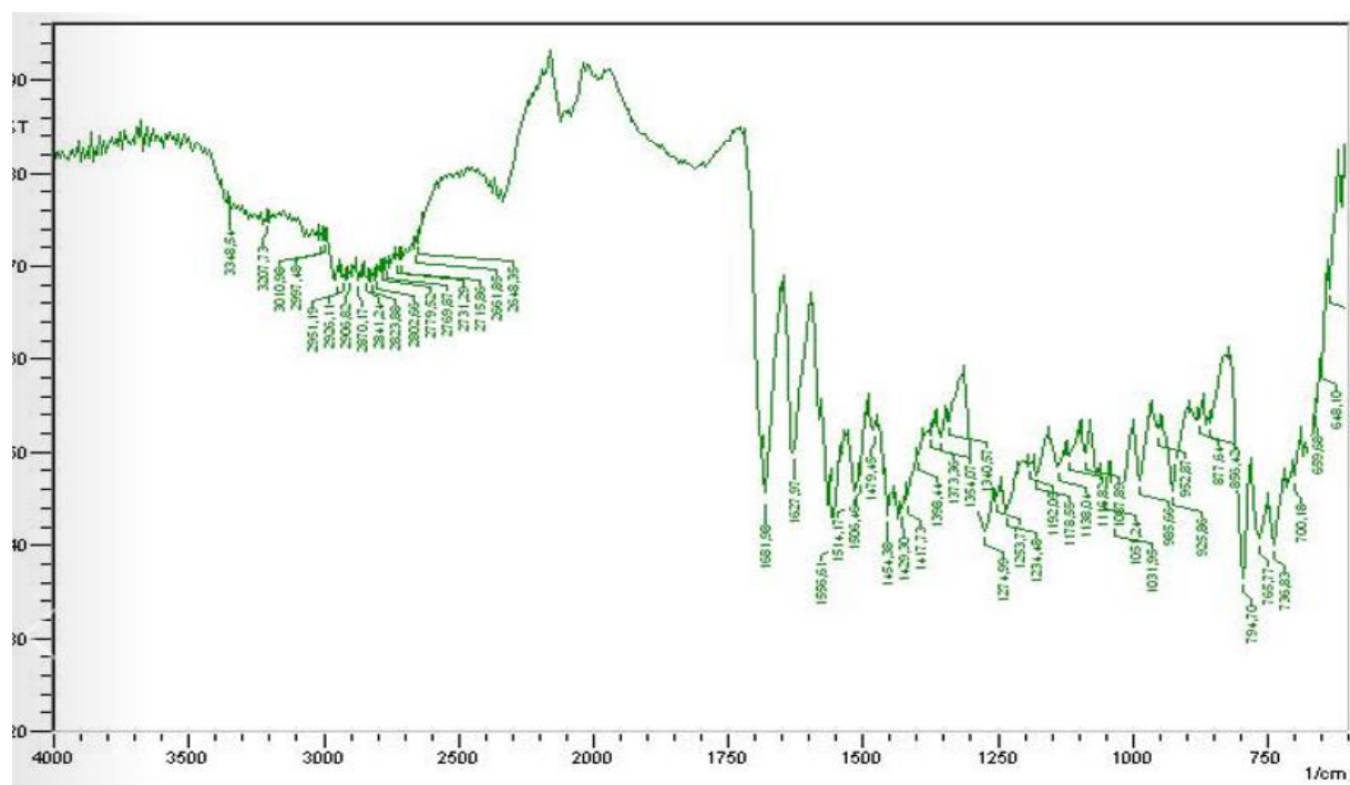
Figure S29. IR spectrum of compound 3h
