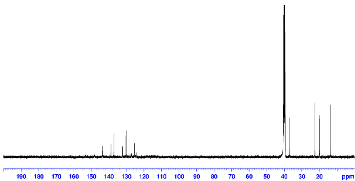
Figure S27. ^{13}\text{C} -NMR spectrum of compound 3g
