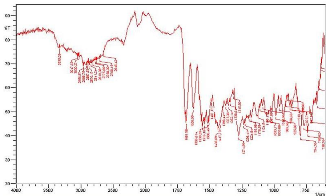
Figure S17. IR spectrum of compound 3e
