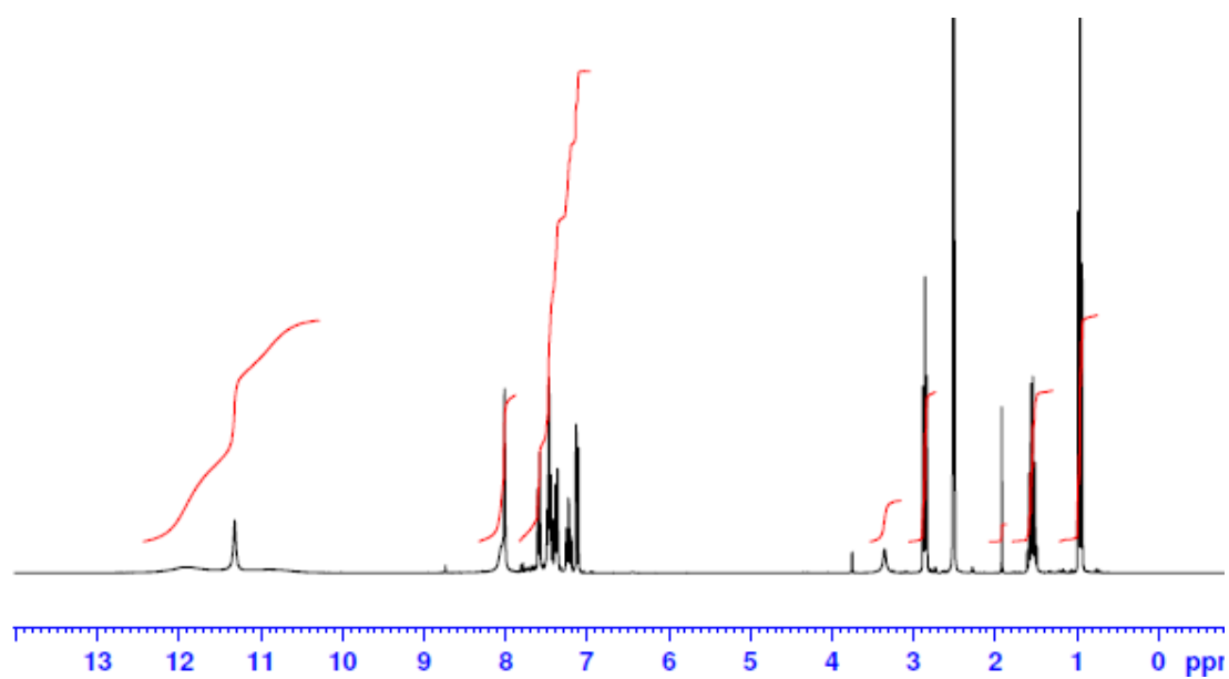
Figure S10. ^1\text{H} -NMR spectrum of compound 3c
