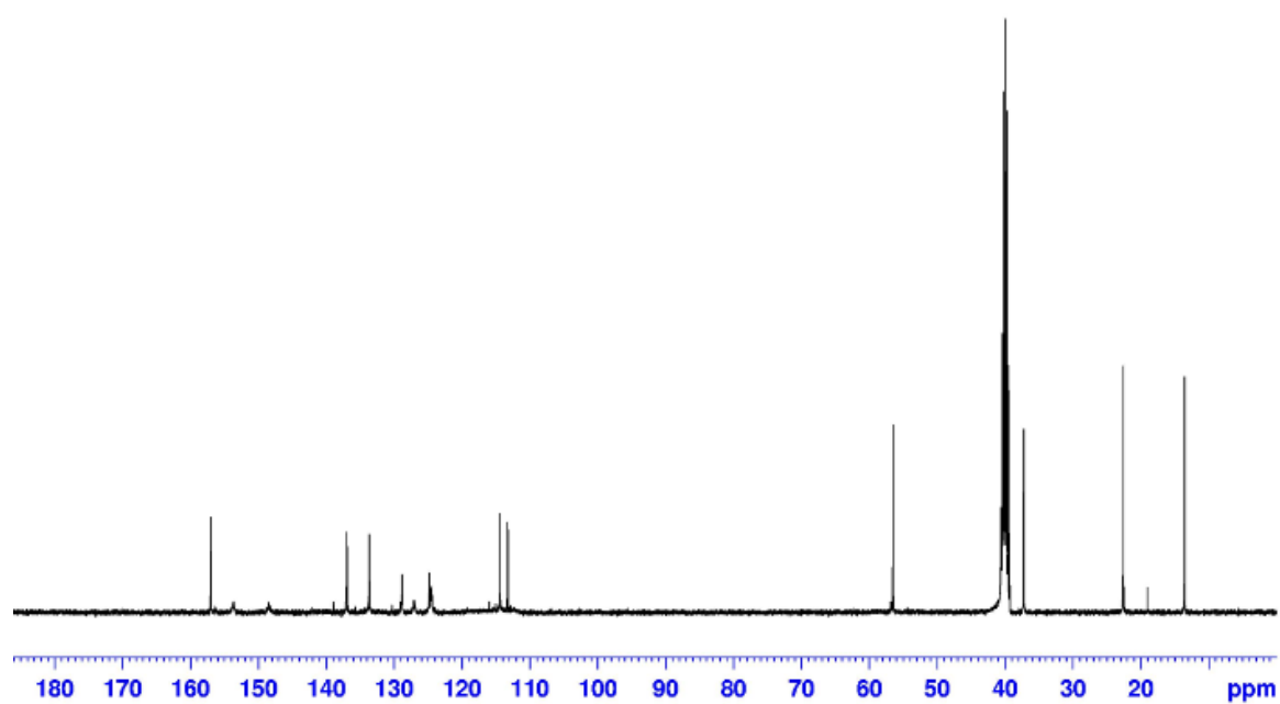
Figure S31. ^{13}\text{C} -NMR spectrum of compound 3h
