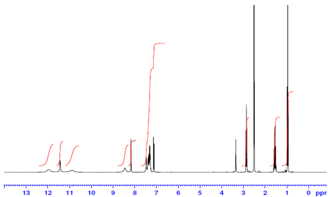
Figure S14. ^1\text{H} -NMR spectrum of compound 3d
