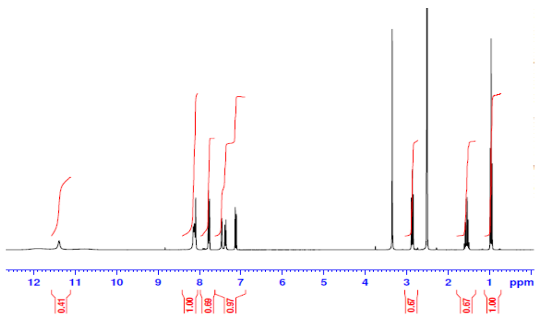
Figure S34. ^1\text{H} -NMR spectrum of compound 3i
