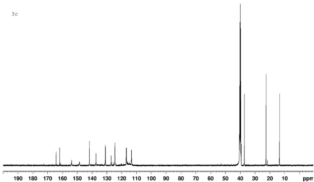
Figure S11. ^{13}\text{C} -NMR spectrum of compound 3c
