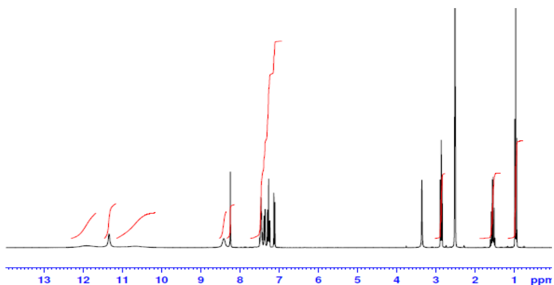
Figure S6. ^1\text{H} -NMR spectrum of compound 3b
