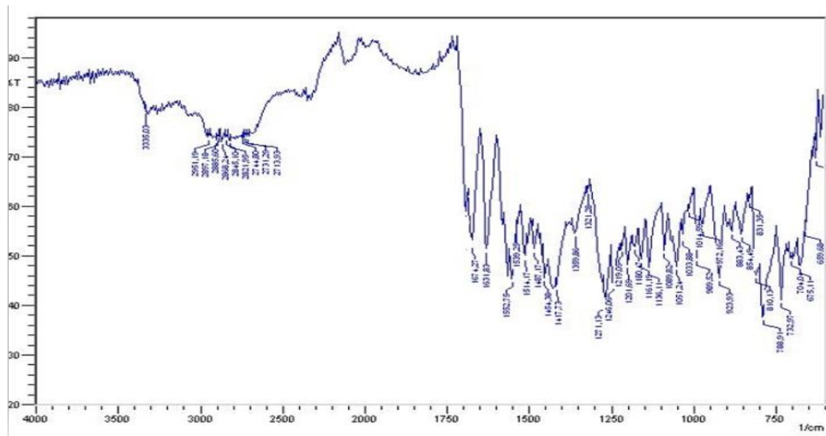
Figure S13. IR spectrum of compound 3d
