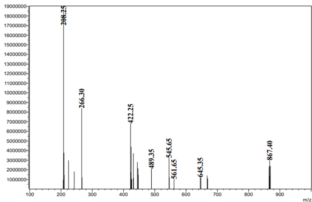
Figure S24. LC/MS spectrum of compound 3f
