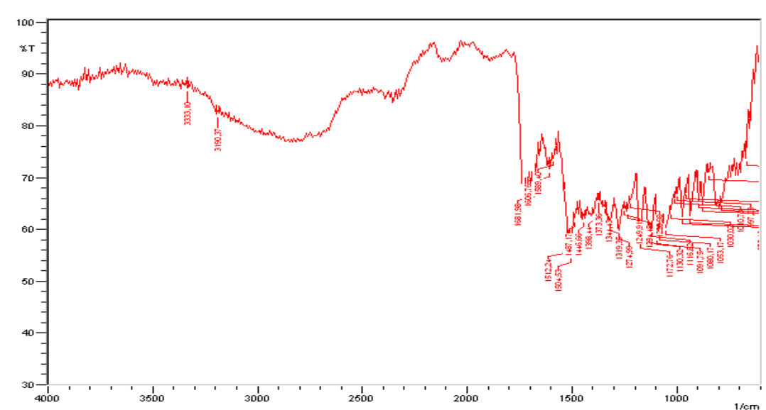
Figure S1. IR spectrum of compound 3a
