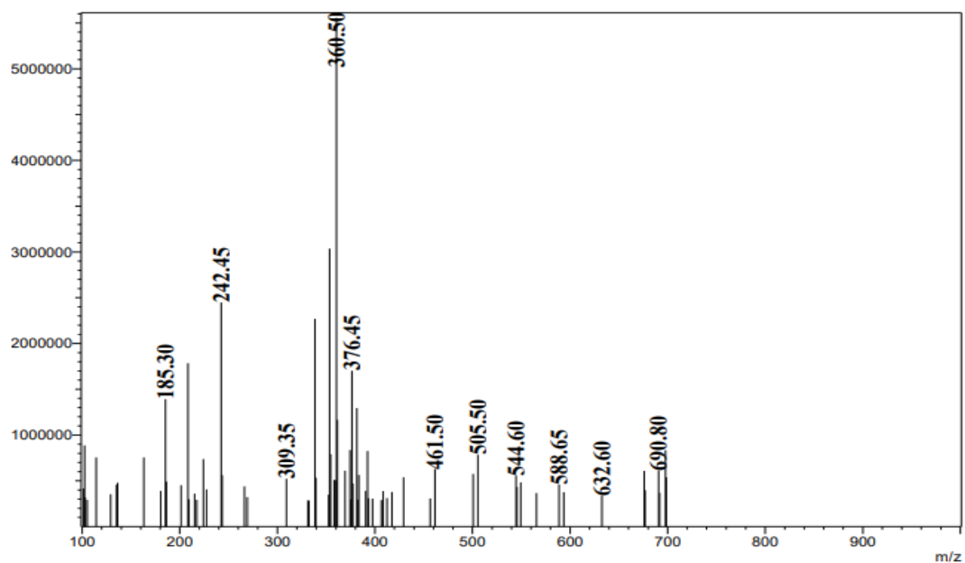
Figure S4. LC/MS spectrum of compound 3a
