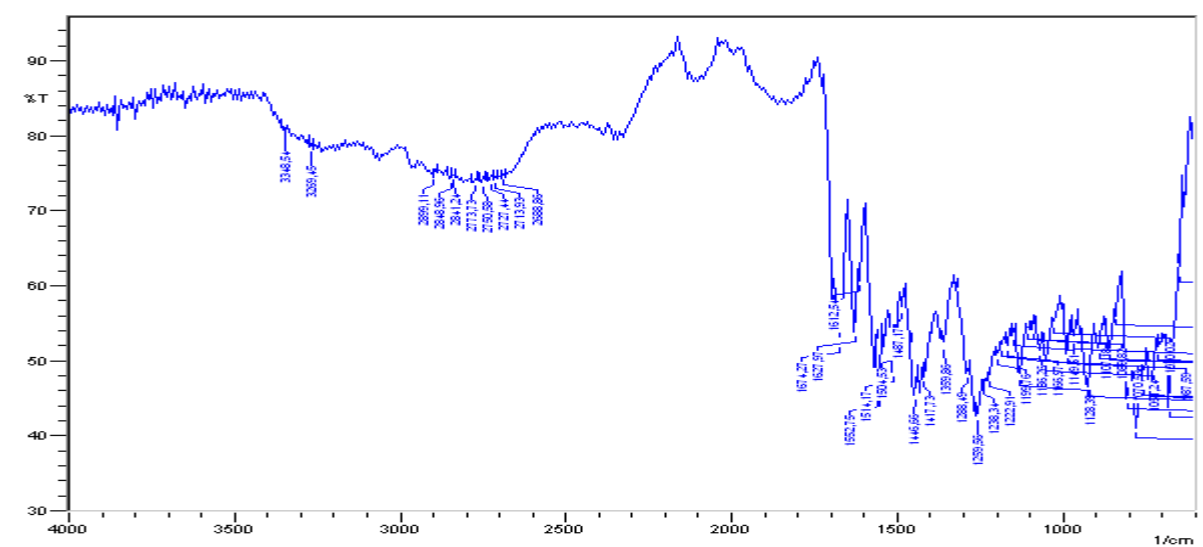
Figure S9. IR spectrum of compound 3c
