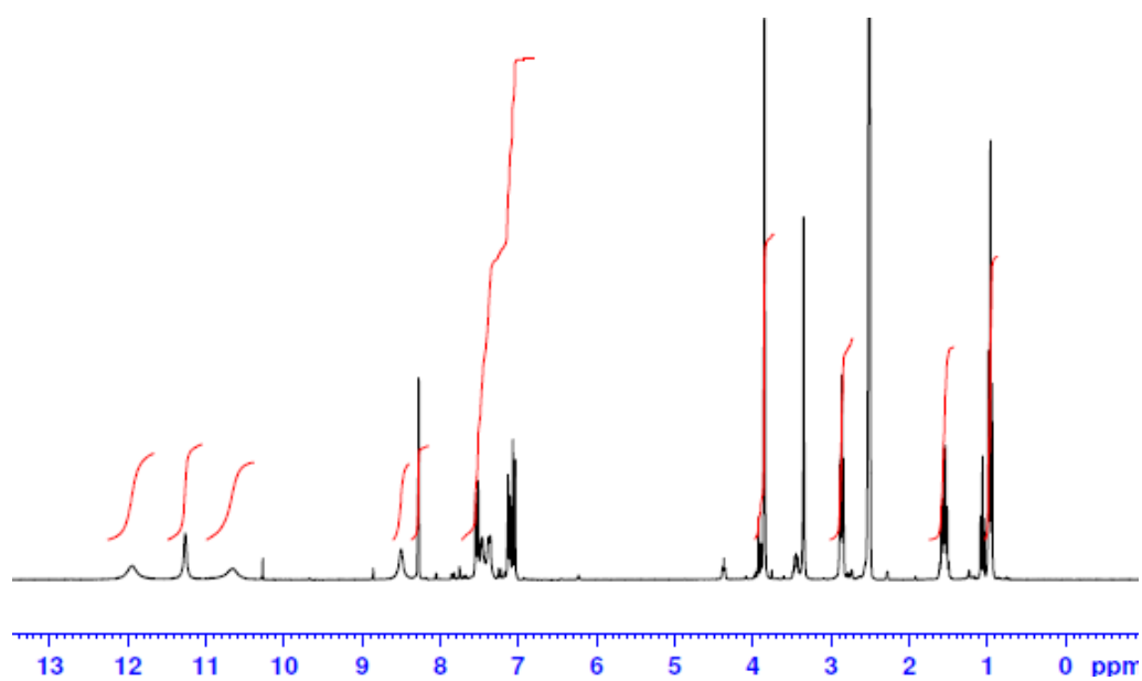
Figure S30. ^1\text{H} -NMR spectrum of compound 3h
