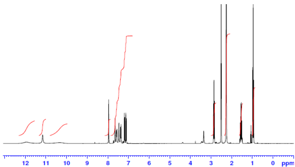
Figure S26. ^1\text{H} -NMR spectrum of compound 3g
