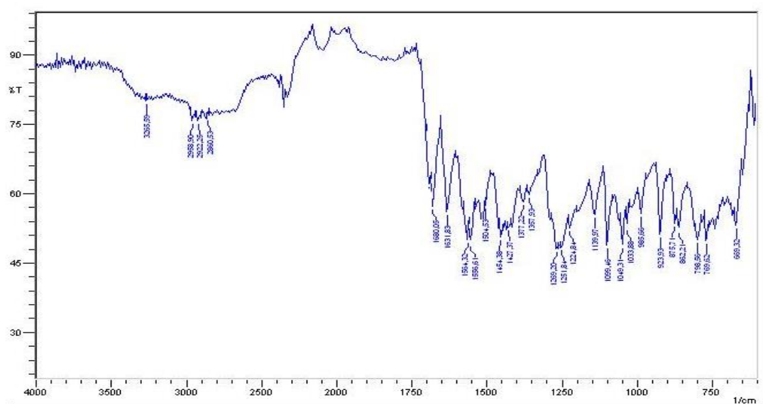
Figure S21. IR spectrum of compound 3f
