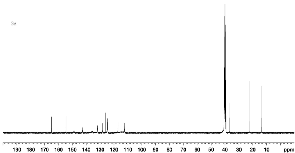
Figure S3. ^{13}\text{C} -NMR spectrum of compound 3a
