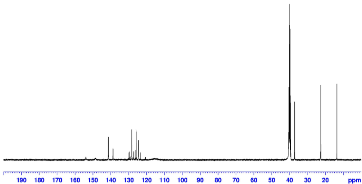
Figure S35. ^{13}\text{C} -NMR spectrum of compound 3i
