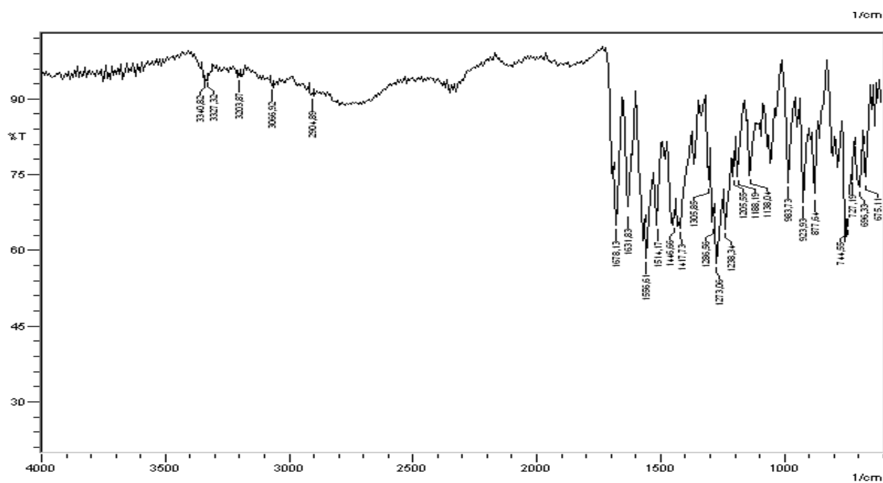
Figure S5. IR spectrum of compound 3b
