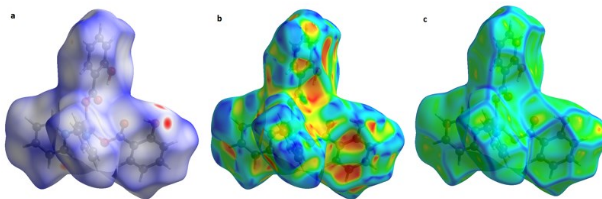
Fig. S1. Hirshfeld surface of molecule 2 a) plotted over d_{\text{norm}} in the range from -0.177 to +1.520 arbitrary units; b) plotted over shape-index property (range from -1.000 to 1.000 ), and c) plotted over curvedness (range from -4.000 to 0.400 ).
