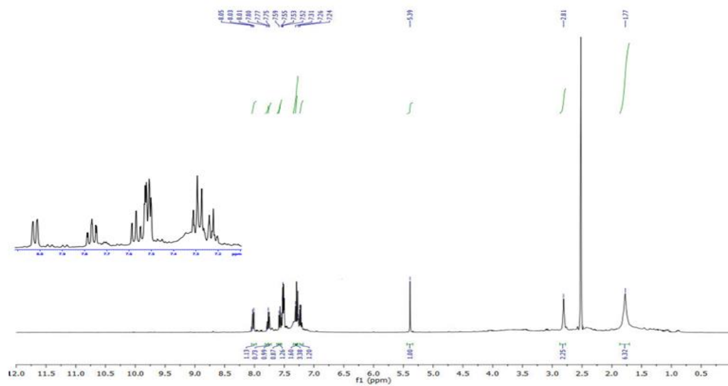
1 H NMR spectrum of 8a
