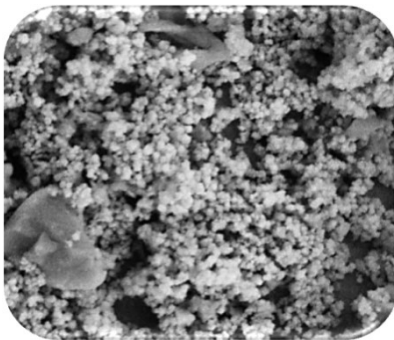
Na-MnO 2
