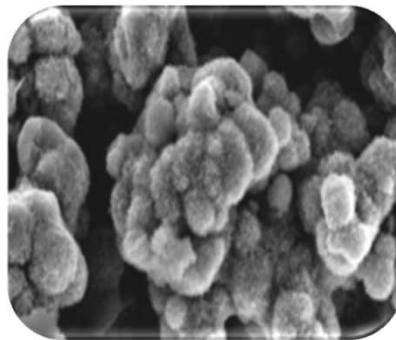
Cocoon-MnO 2
