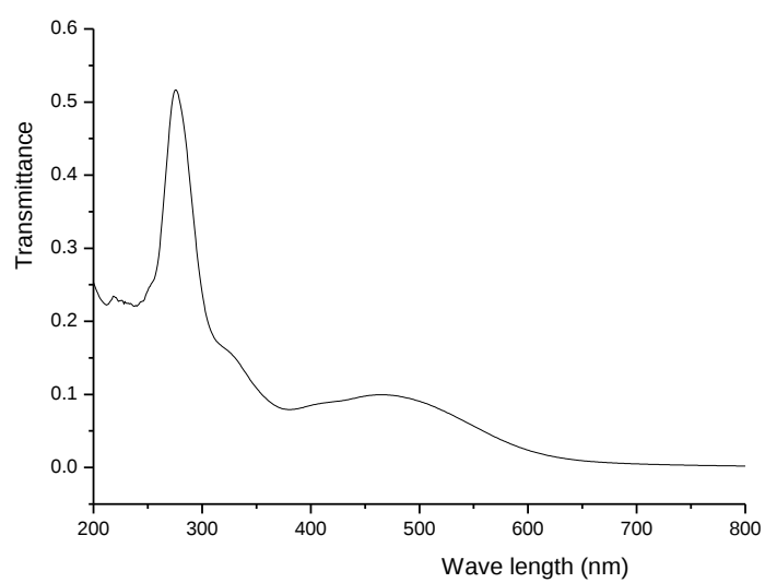
Fig. S5. UV-Vis spectrum of complex 1.
