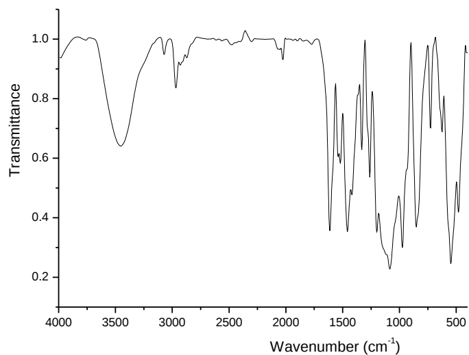
Fig. S2. IR spectrum of complex 1.
