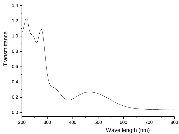
Fig. S6. UV-Vis spectrum of complex 2.
