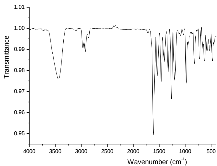
Fig. S3. IR spectrum of complex 2.
