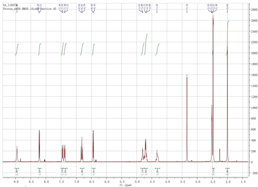
Fig. 7. ^1\text{H} NMR spectrum of complex 1.
