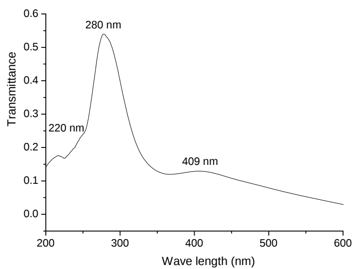
Fig. 6. UV–Vis spectrum of complex 2.
