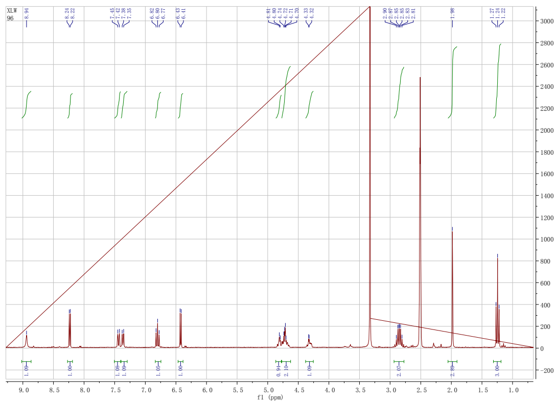
Fig. 8. ^1\text{H} NMR spectrum of complex 2.
