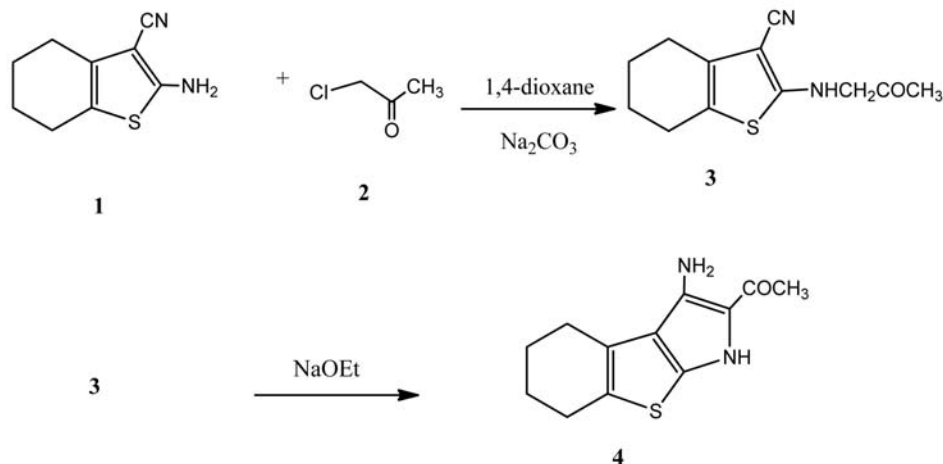
Shema 1. Synthesis of compounds 3 and 4 .
