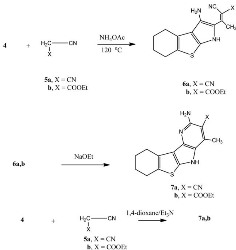
Shema 2. Synthesis of compounds 6a,b and 7a,b .
