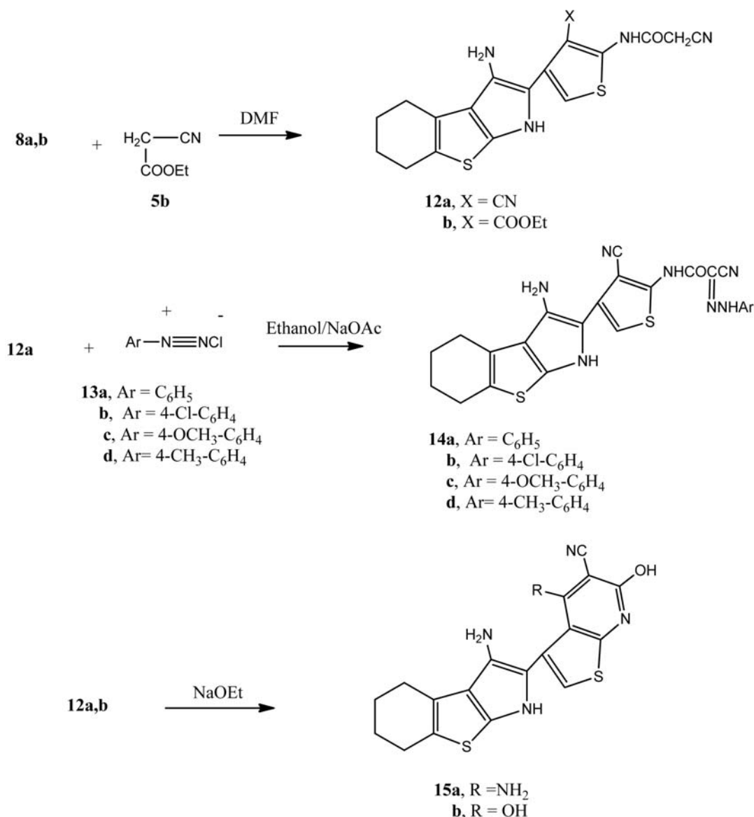
Scheme 4. Synthesis of compounds 12a,b-15a,b .
