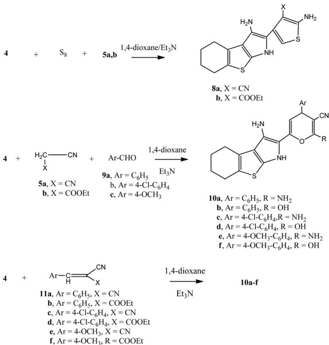
Scheme 3. Synthesis of compounds 8a,b and 10a-f .
