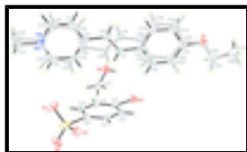
Fig. 1. The molecular structure of the title compound, with 50% probability displacement ellipsoids and the atom-numbering scheme. Open bonds show the minor component.
