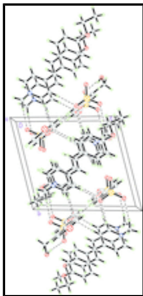
Fig. 2. The crystal packing of the major component of the title compound viewed down the a axis. O—H...O hydrogen bonds and C—H...O weak interactions are shown as dashed lines.
