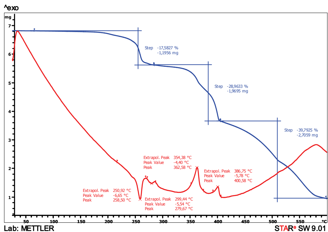
Figure S8. TG/DTA curve of [Cd(N 3 ) 2 (pia)] n ·H 2 O (4).
