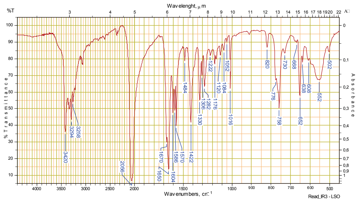
Figure S4. IR spectrum of [Cd(N_3)_2(pia)]_n ( 4 ).
