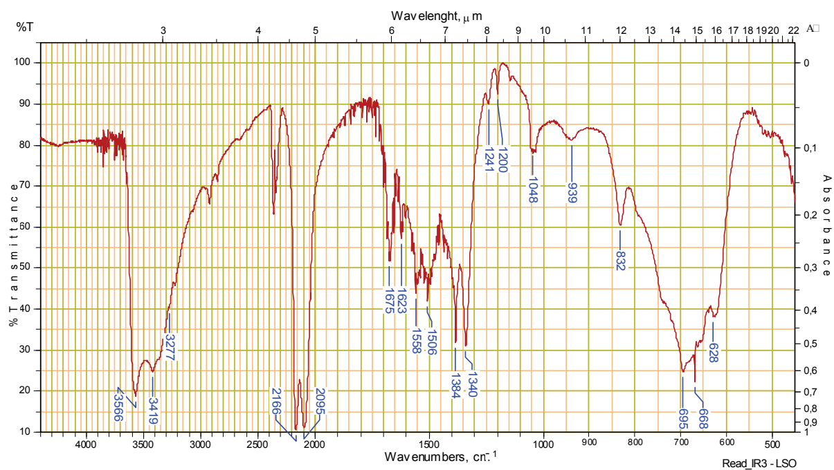
Figure S3. IR spectrum of [Zn(N_3)_2(pia)_2] ( 3 ).
