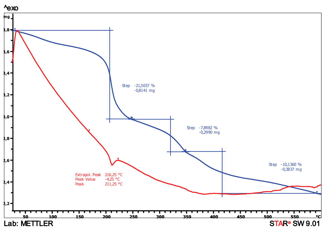
Figure S7. TG/DTA curve of [Zn(N 3 ) 2 (pia) 2 ] (3).
