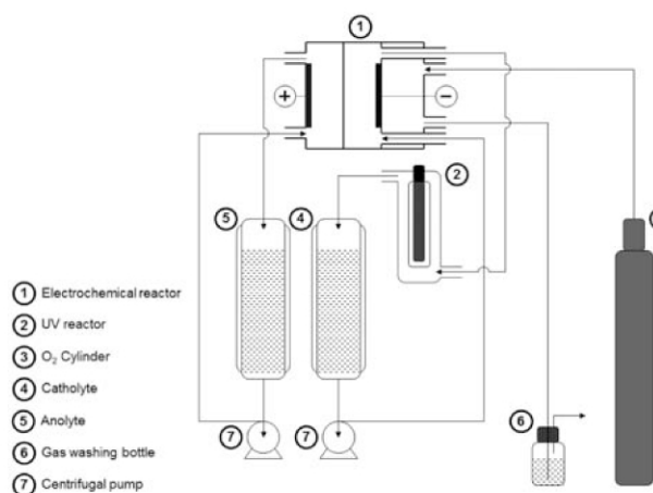
Figure 1. Schematic of the used laboratory setup.
